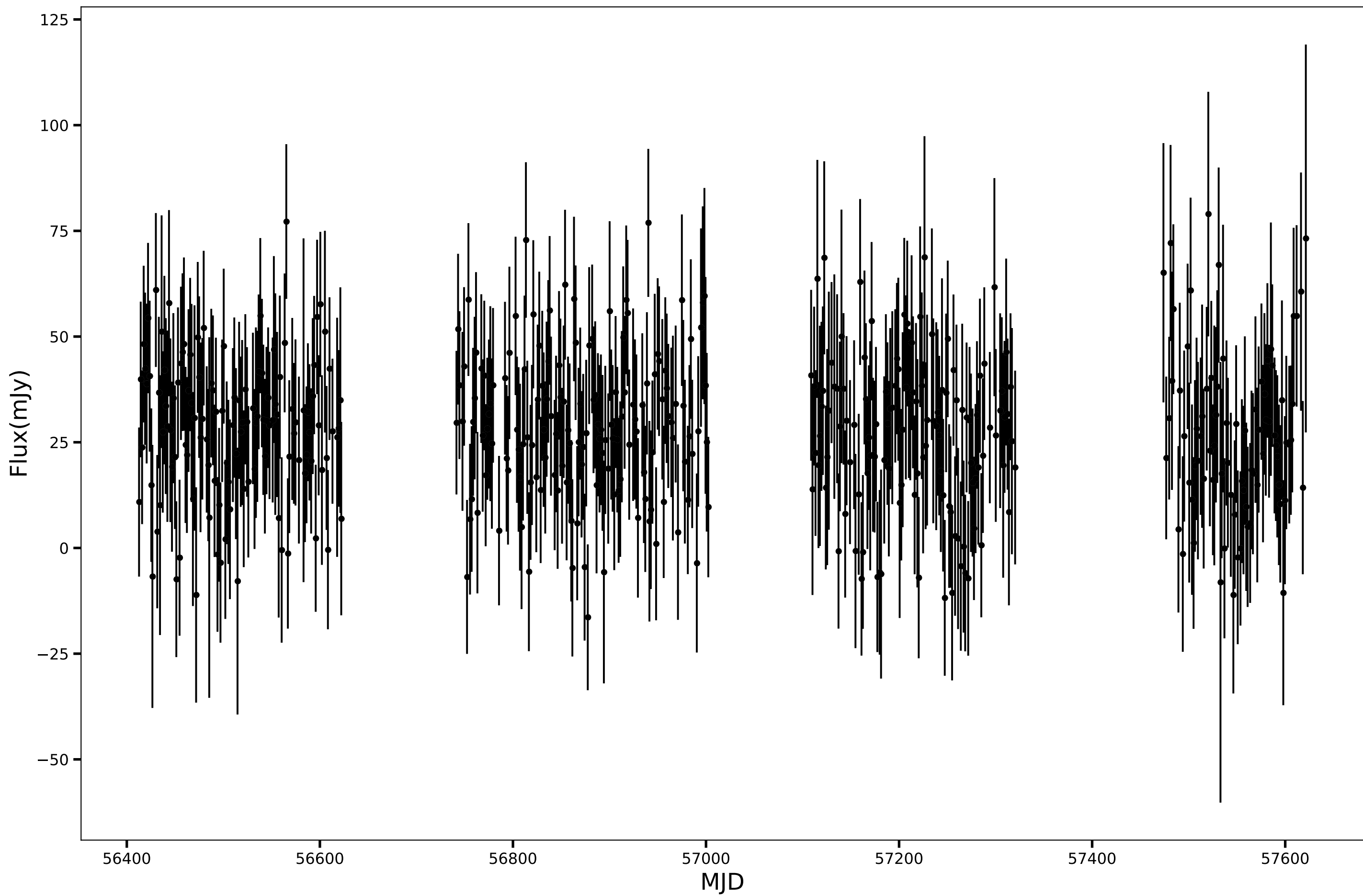
SPT-SJ003725-5917.9, RA=9.3572d, DEC=-59.2997d, mean_flux=27.91 (mJy), 90GHz
