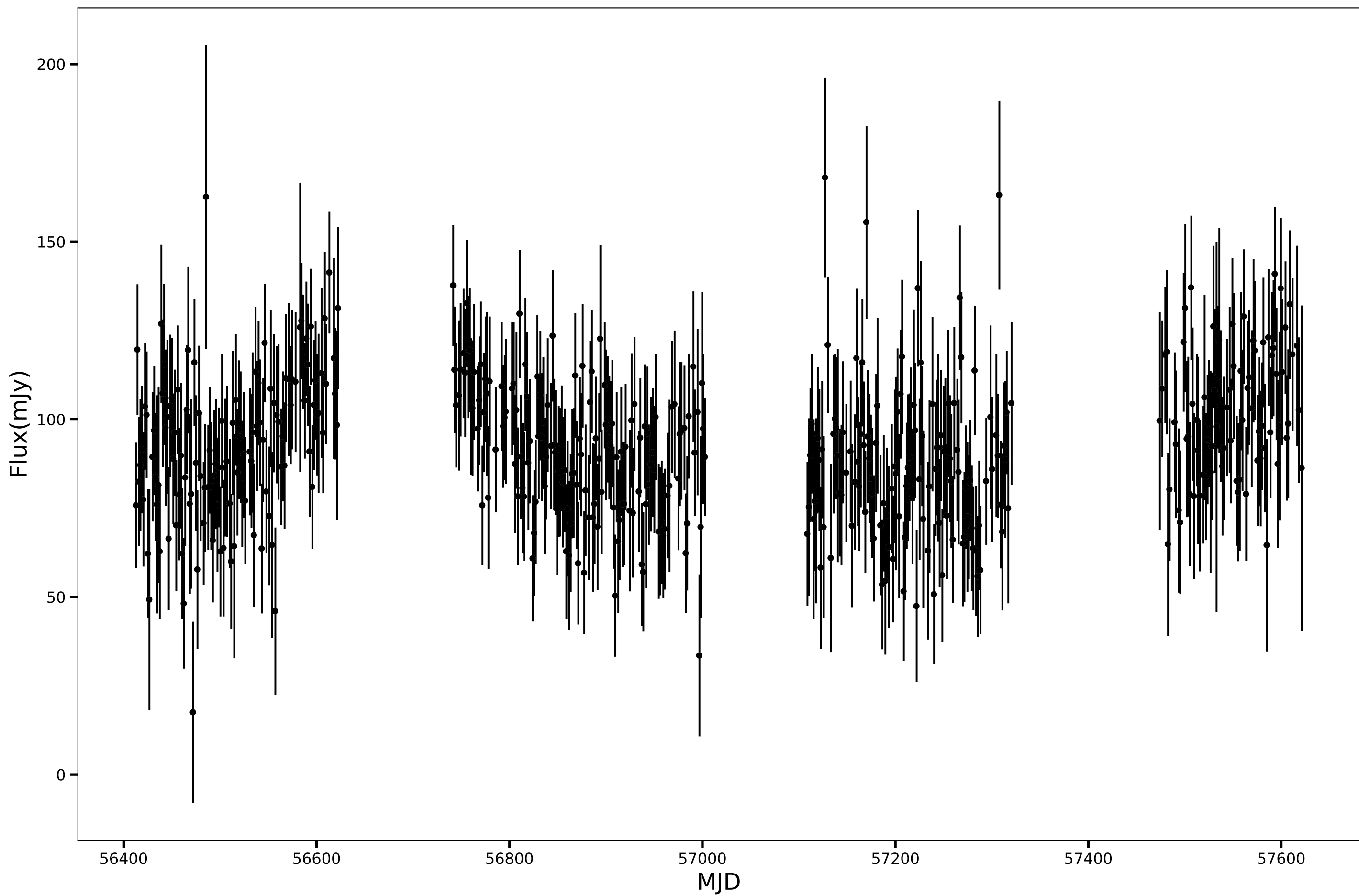
SPT-SJ003133-5143.3, RA=7.8913d, DEC=-51.7229d, mean_flux=92.28 (mJy), 90GHz
