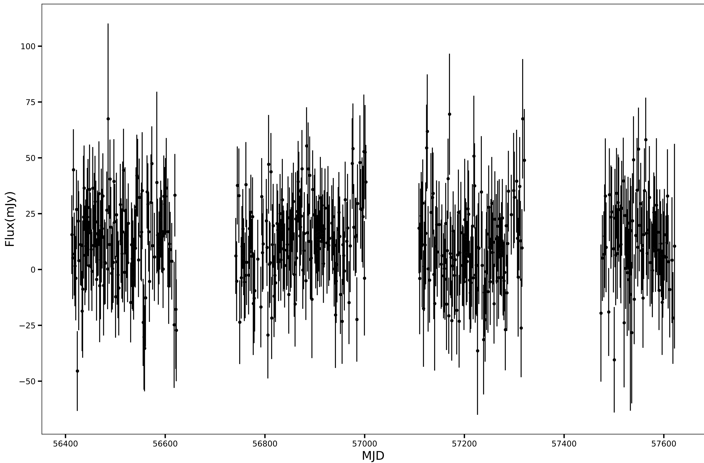
SPT-SJ002736-5409.2, RA=6.9038d, DEC=-54.1545d, mean_flux=12.08 (mJy), 90GHz
