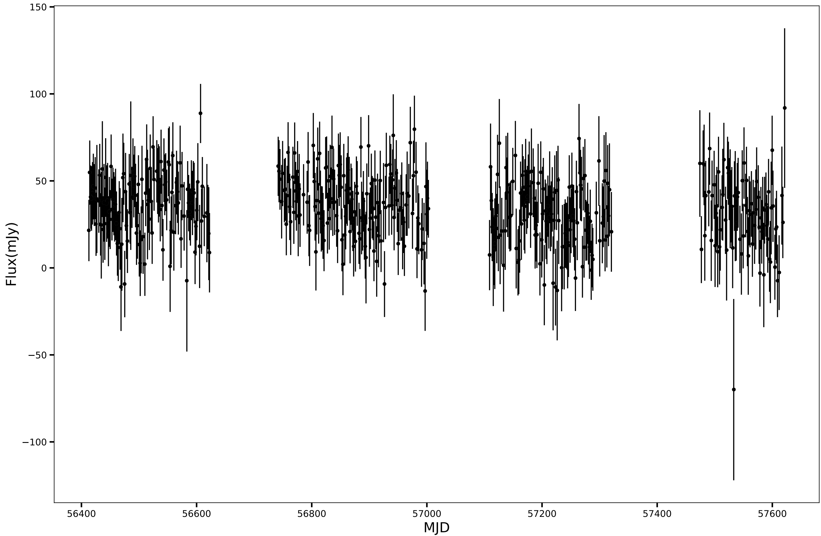
SPT-SJ002510-5427.5, RA=6.2927d, DEC=-54.4599d, mean_flux=33.71 (mJy), 90GHz
