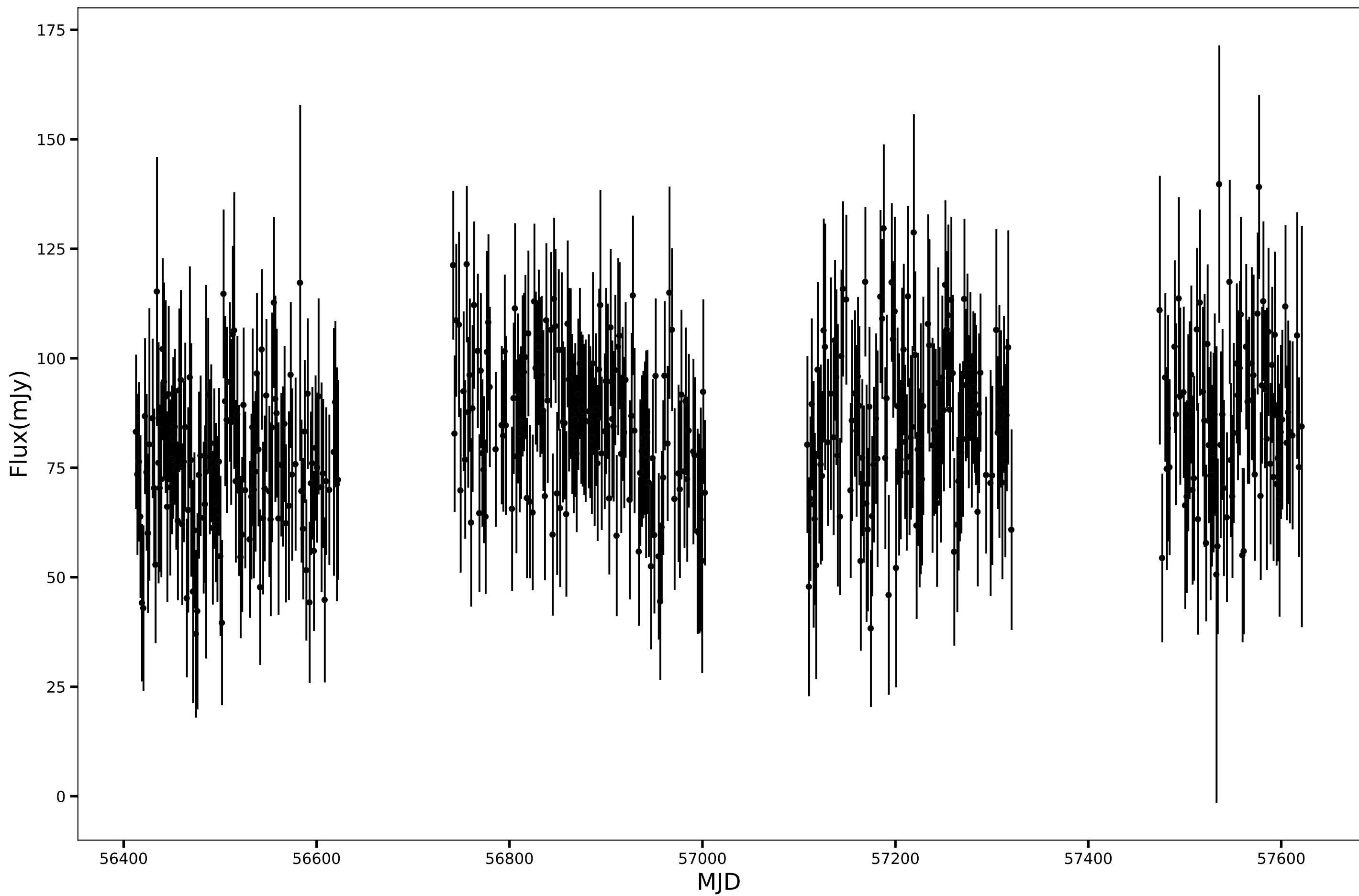
SPT-SJ002302-5650.1, RA=5.7600d, DEC=-56.8355d, mean_flux=83.07 (mJy), 90GHz
