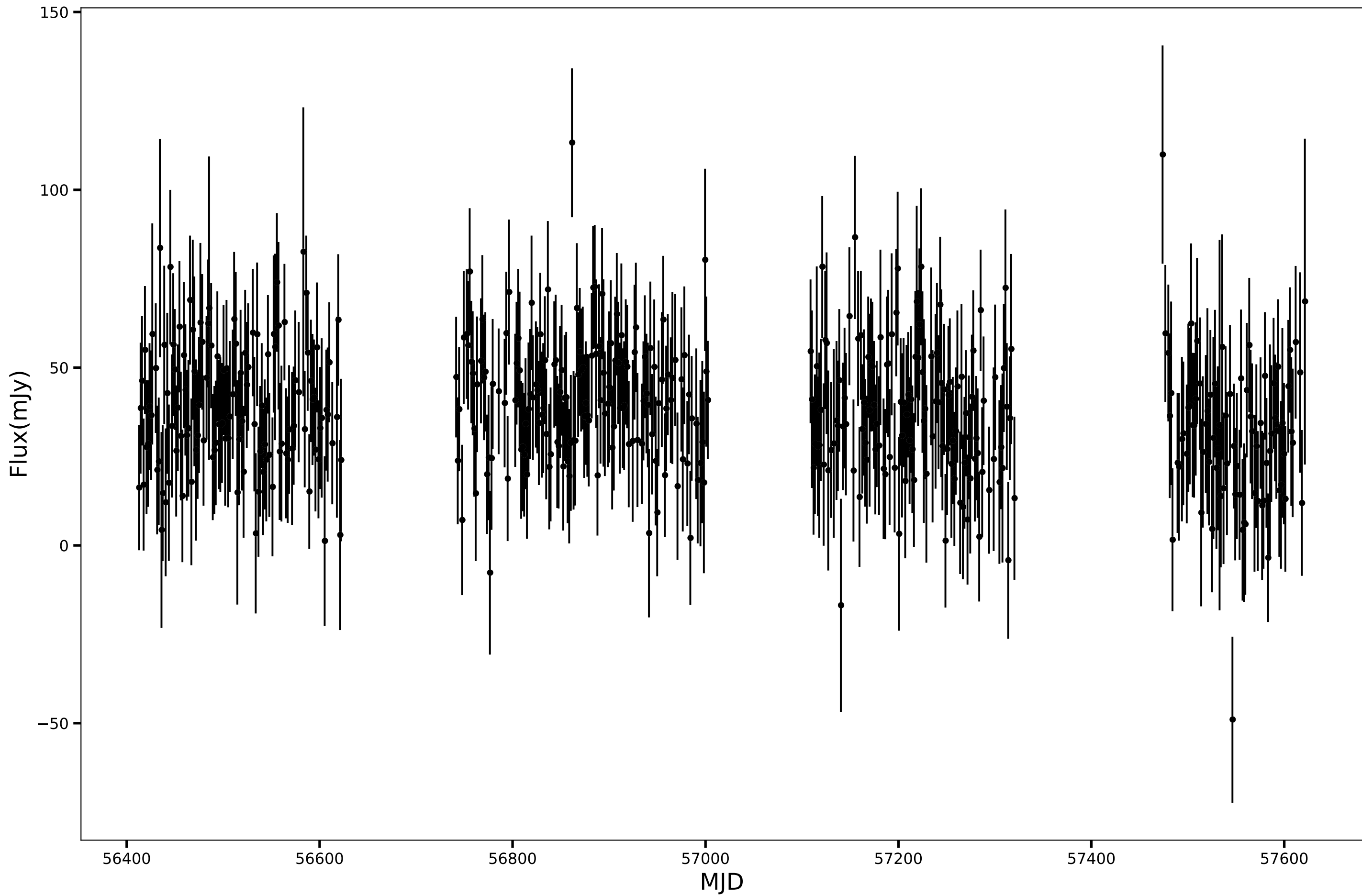
SPT-SJ002233-5153.2, RA=5.6387d, DEC=-51.8871d, mean_flux=37.93 (mJy), 90GHz
