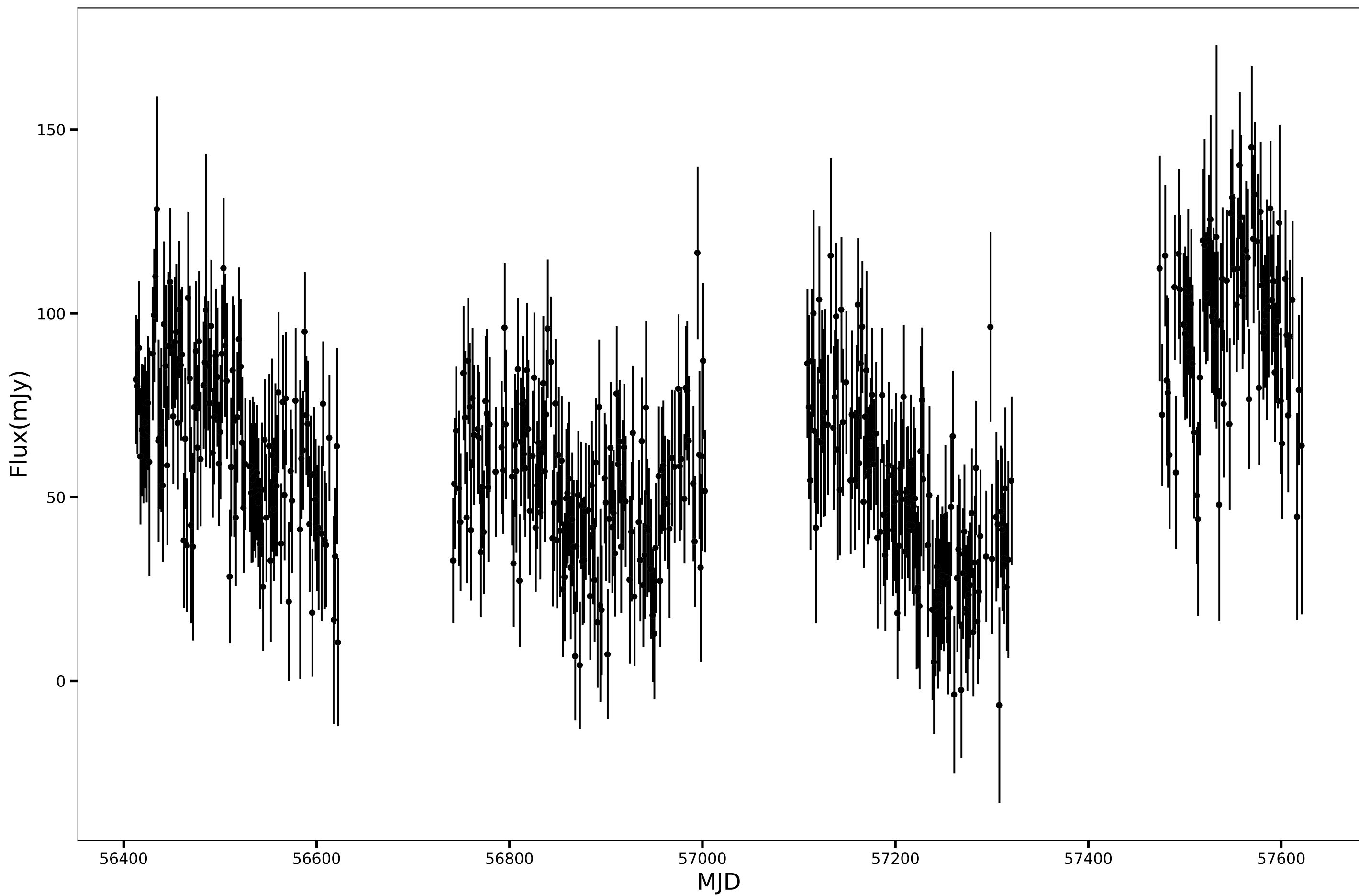
SPT-SJ001926-5641.7, RA=4.8610d, DEC=-56.6961d, mean_flux=63.41 (mJy), 90GHz
