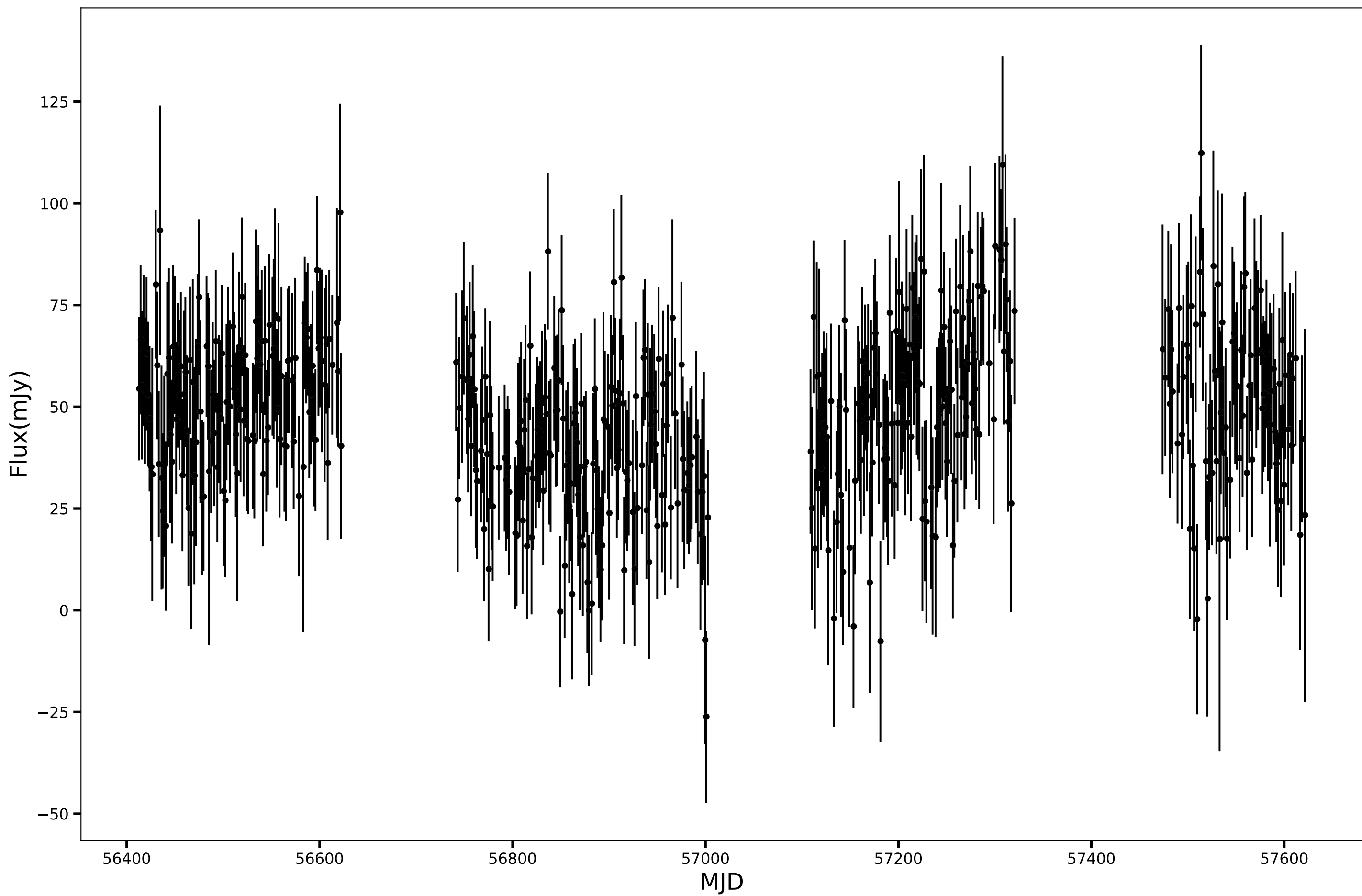
SPT-SJ001426-5638.4, RA=3.6122d, DEC=-56.6404d, mean_flux=47.52 (mJy), 90GHz
