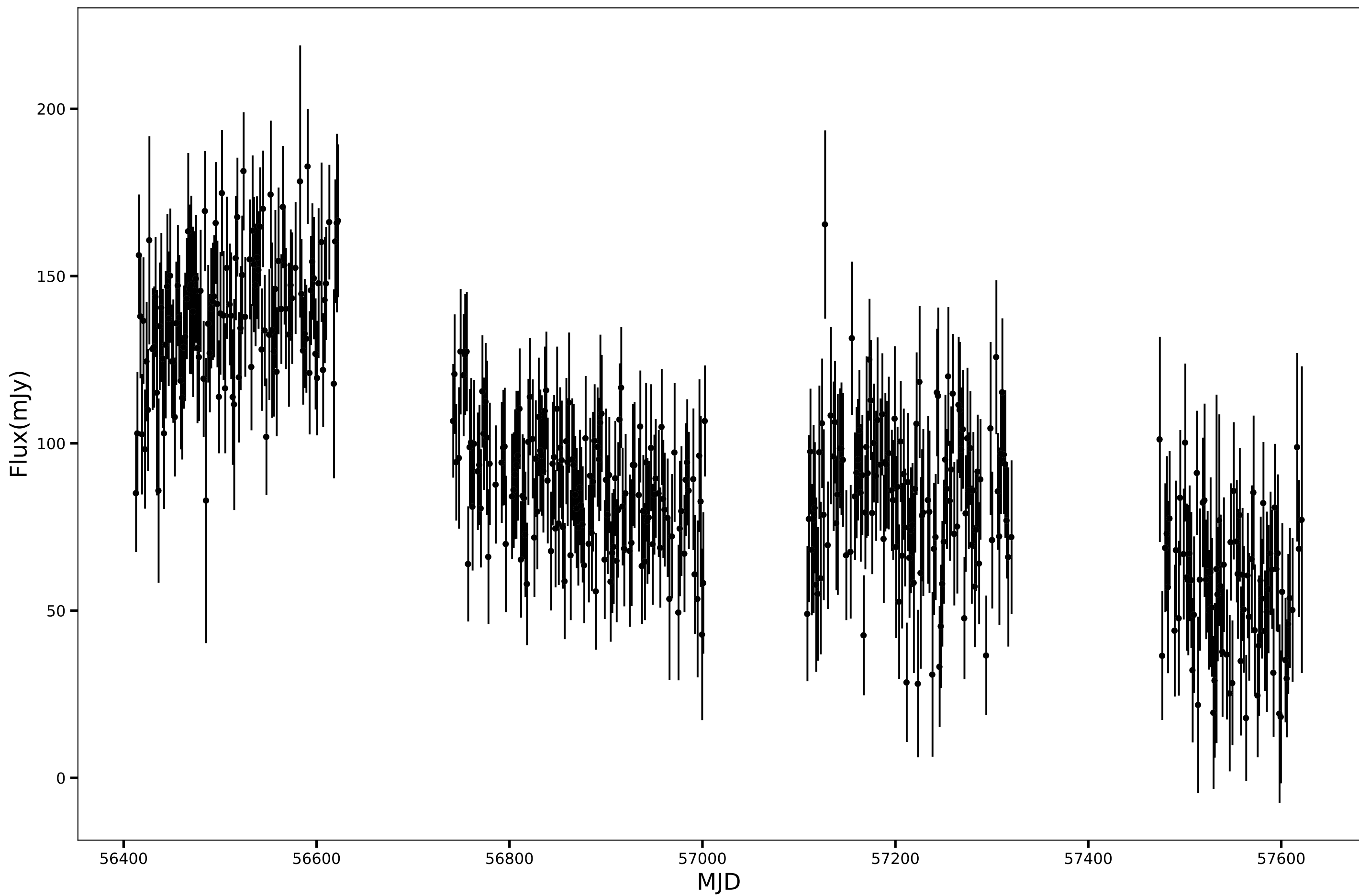
SPT-SJ001324-5005.2, RA=3.3516d, DEC=-50.0877d, mean_flux=94.67 (mJy), 90GHz
