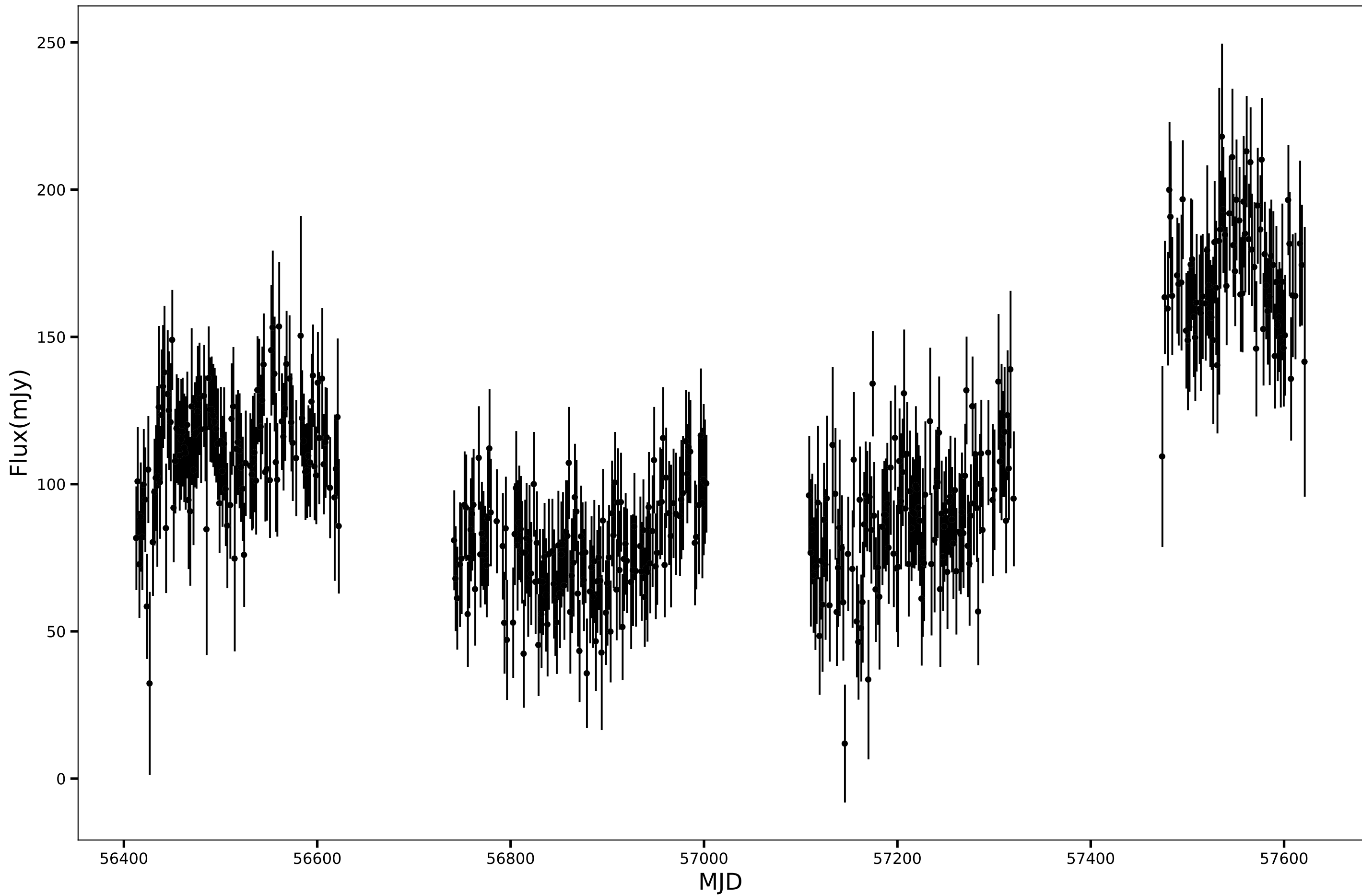
SPT-SJ000800-5243.6, RA=2.0027d, DEC=-52.7277d, mean_flux=105.41 (mJy), 90GHz
