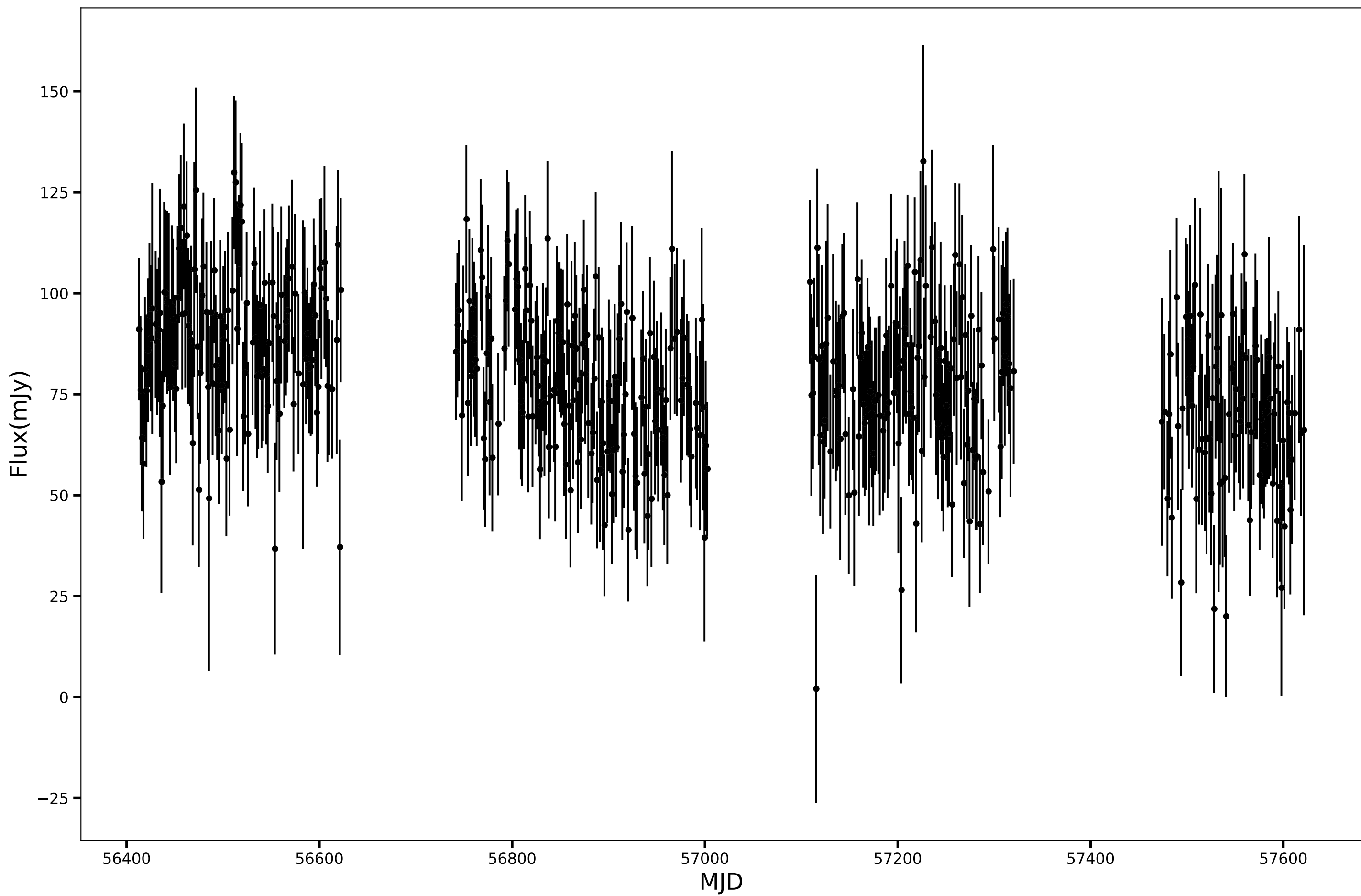
SPT-SJ000719-6113.2, RA=1.8315d, DEC=-61.2210d, mean_flux=79.04 (mJy), 90GHz
