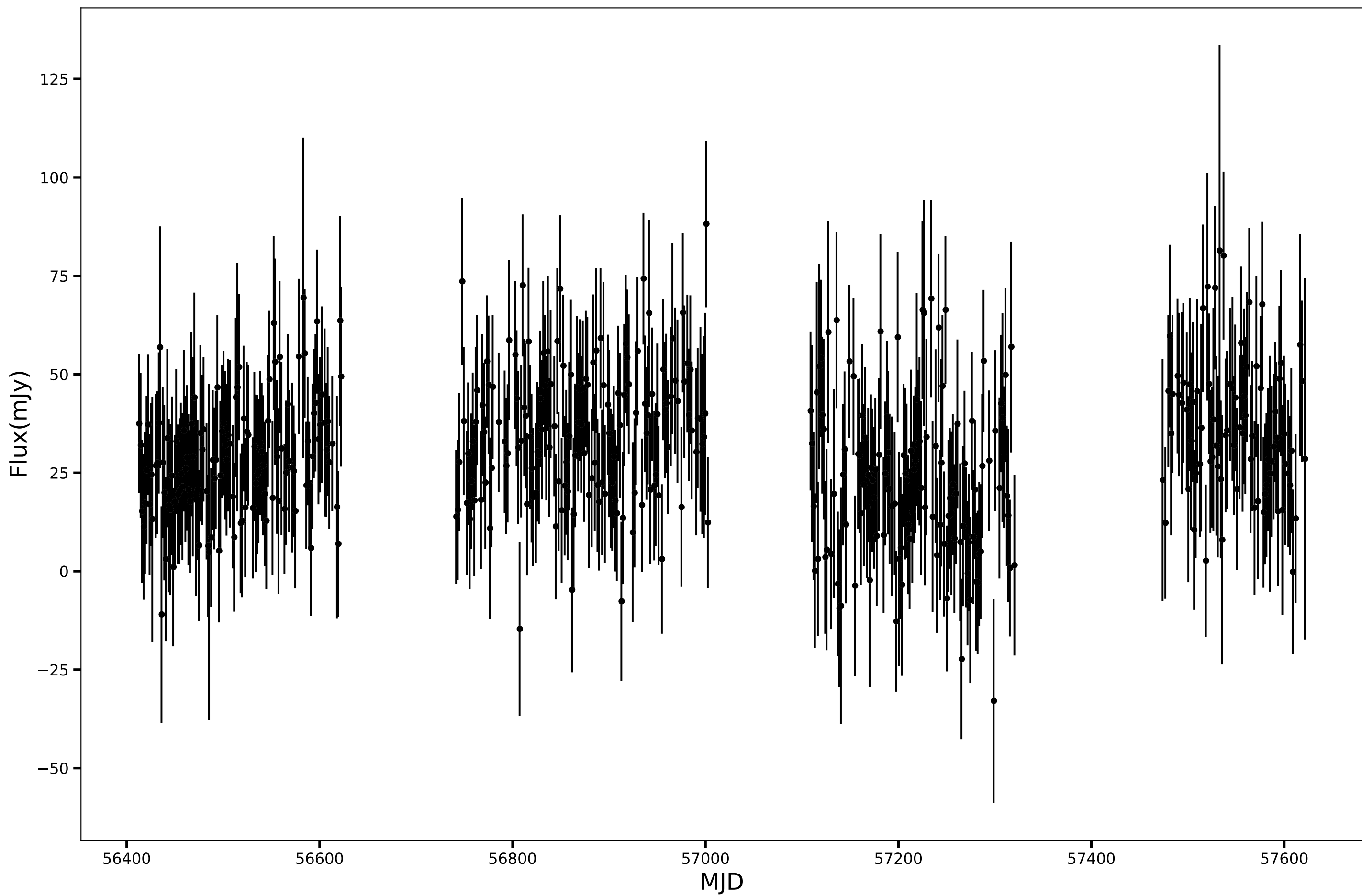
SPT-SJ000303-5529.9, RA=0.7640d, DEC=-55.4997d, mean_flux=30.61 (mJy), 90GHz
