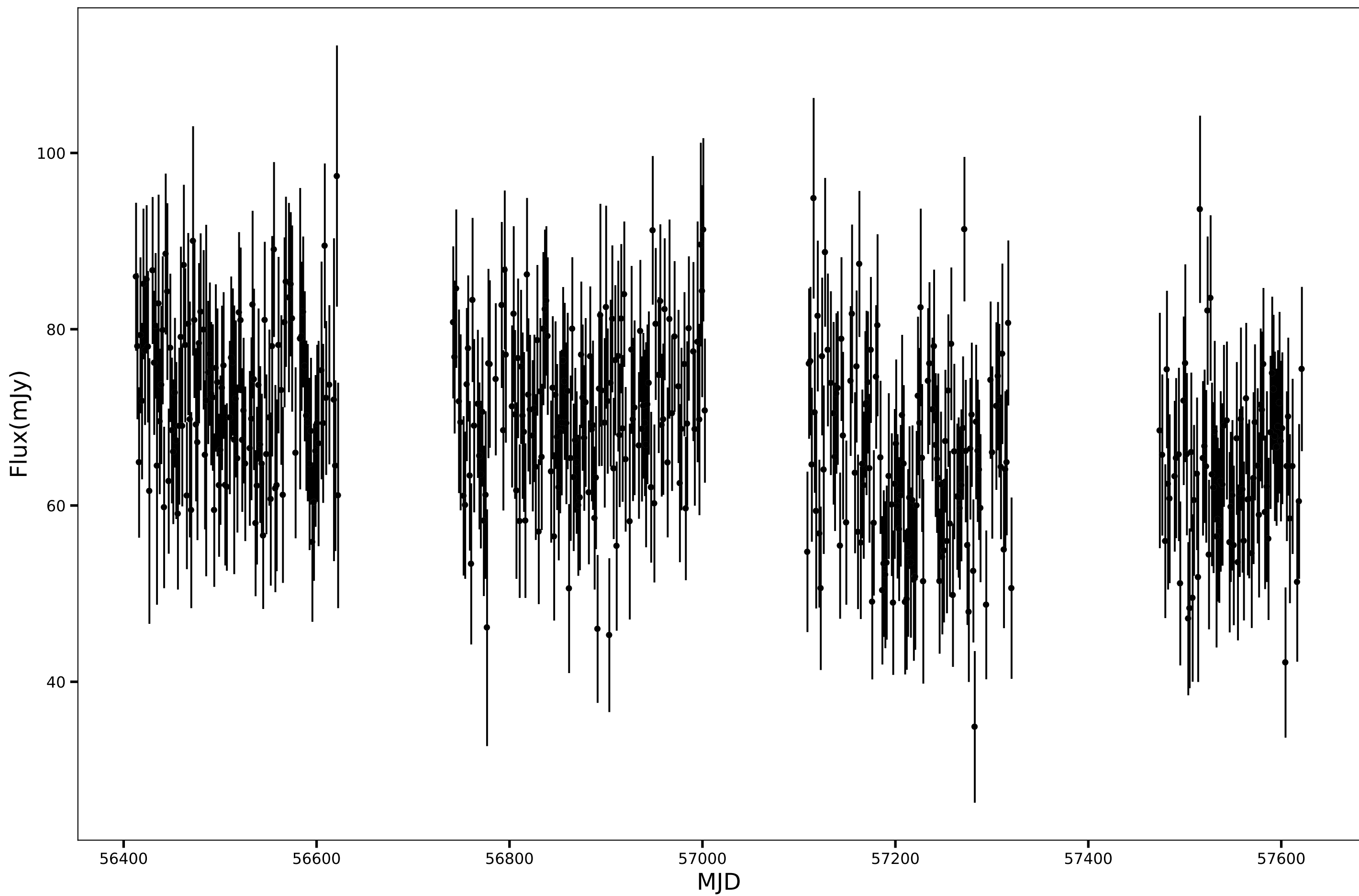
SPT-SJ235920-6057.0, RA=359.8371d, DEC=-60.9500d, mean_flux=68.65 (mJy), 150GHz
