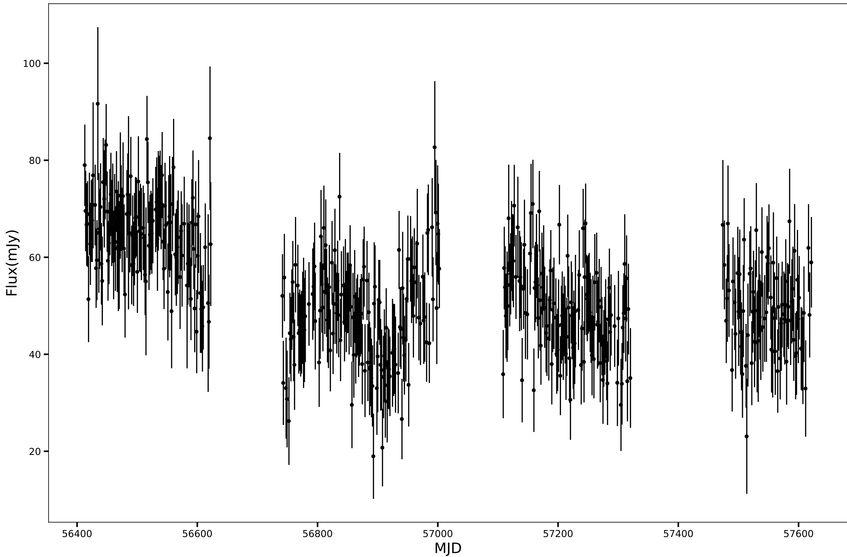
SPT-SJ235903-6055.1, RA=359.7654d, DEC=-60.9192d, mean_flux=52.91 (mJy), 150GHz
