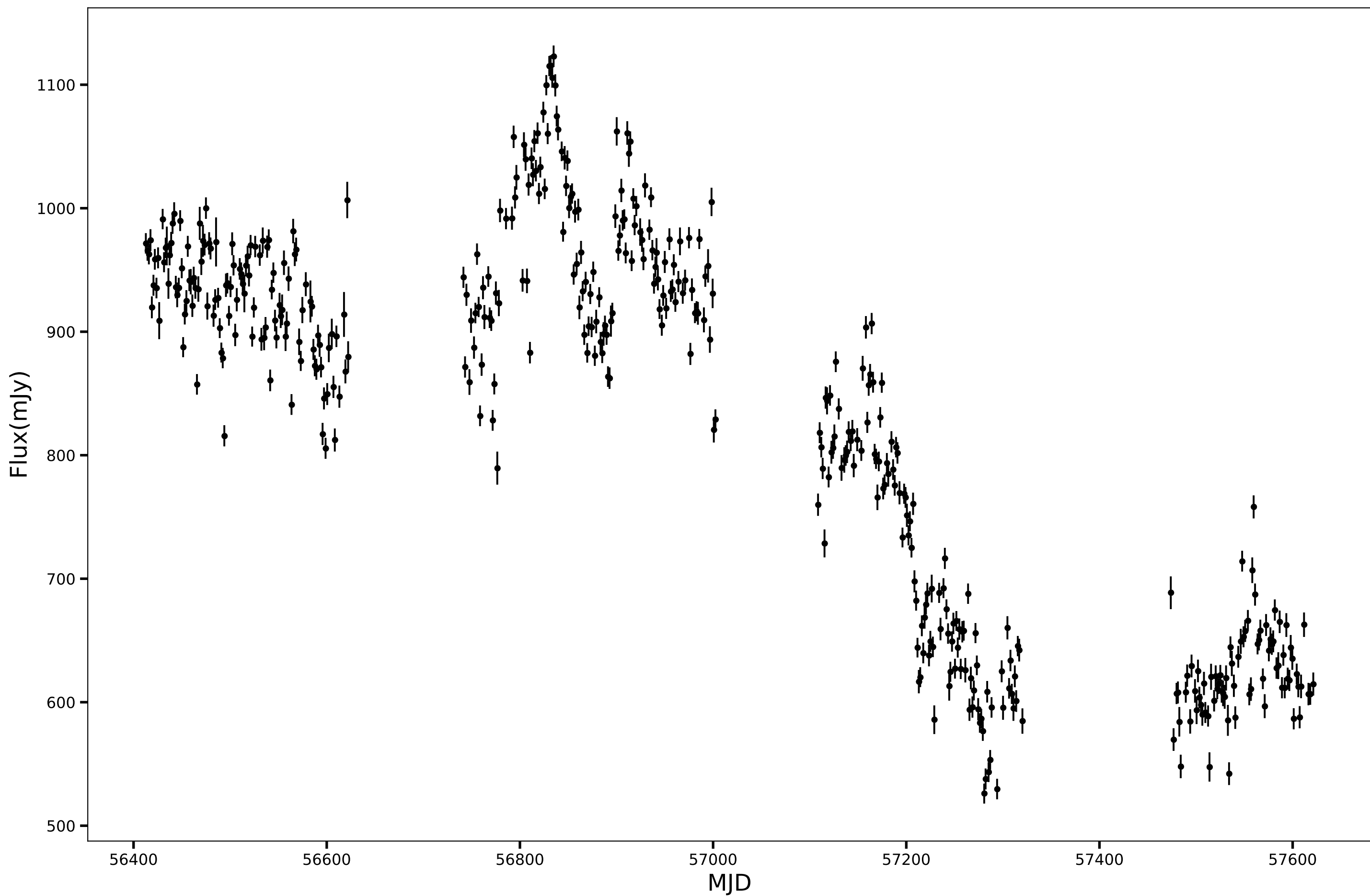
SPT-SJ235753-5311.2, RA=359.4721d, DEC=-53.1877d, mean_flux=829.72 (mJy), 150GHz
