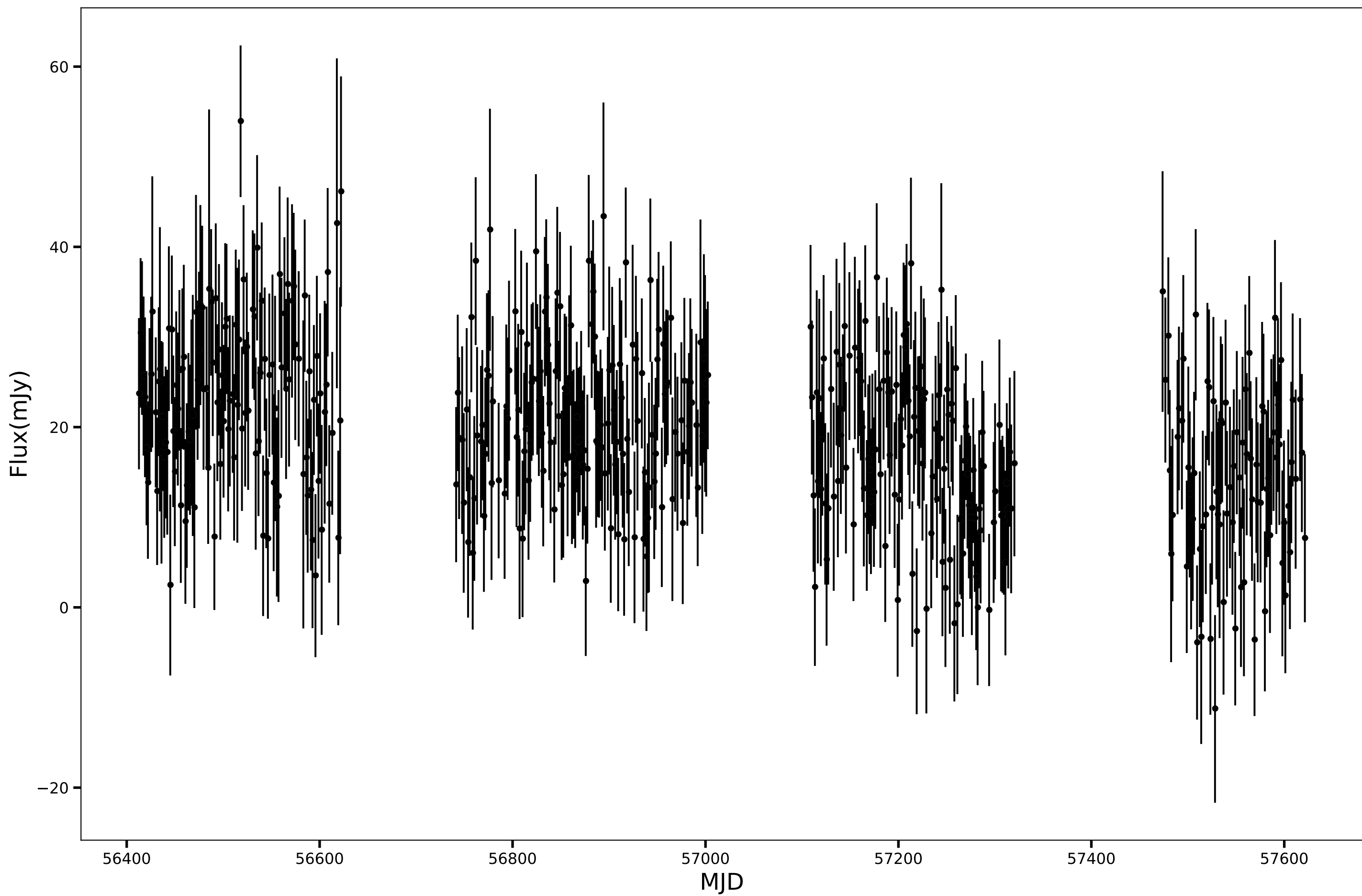
SPT-SJ235322-5857.3, RA=358.3446d, DEC=-58.9559d, mean_flux=19.33 (mJy), 150GHz
