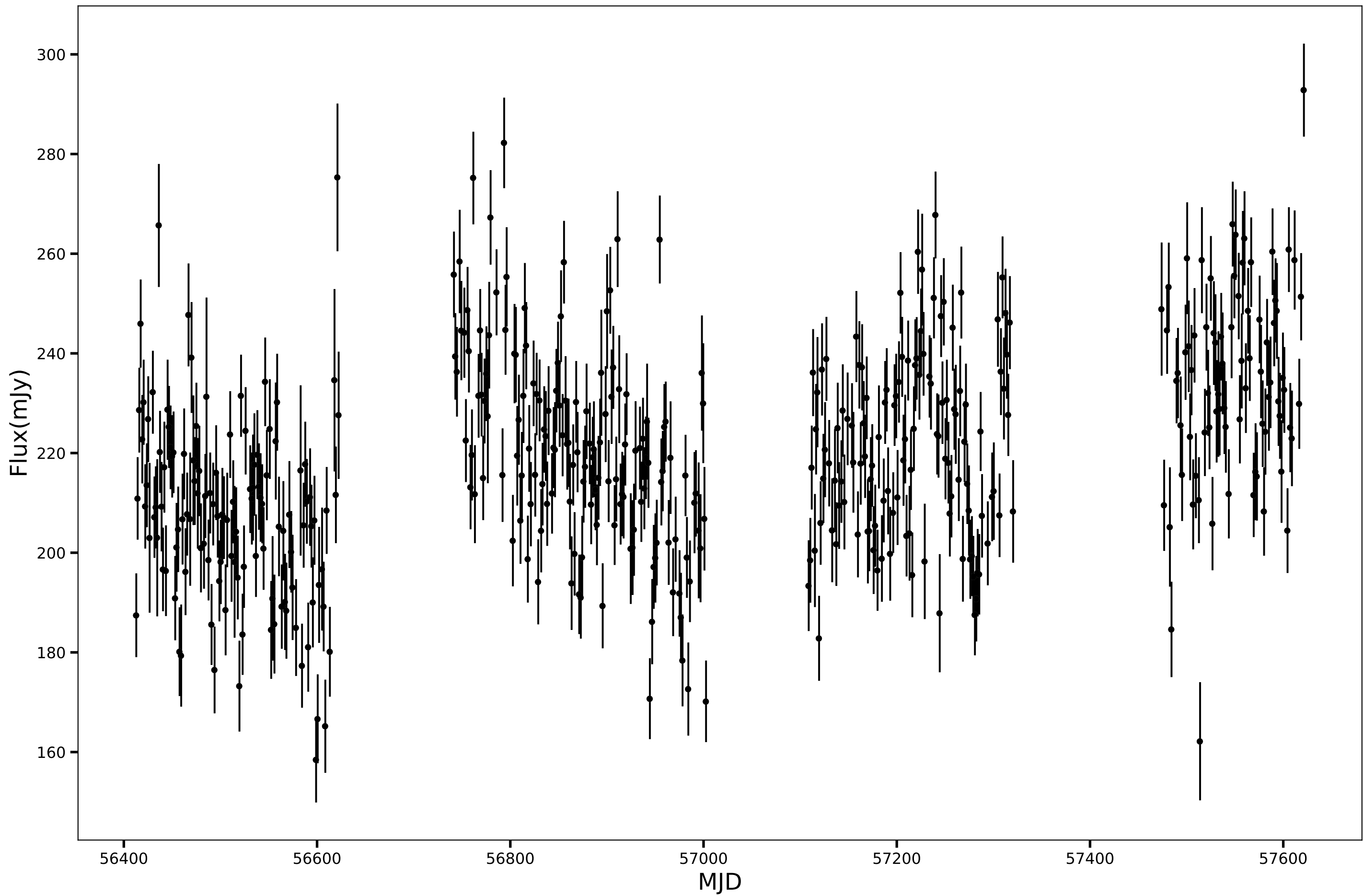
SPT-SJ234925-4932.4, RA=357.3583d, DEC=-49.5408d, mean_flux=219.83 (mJy), 150GHz
