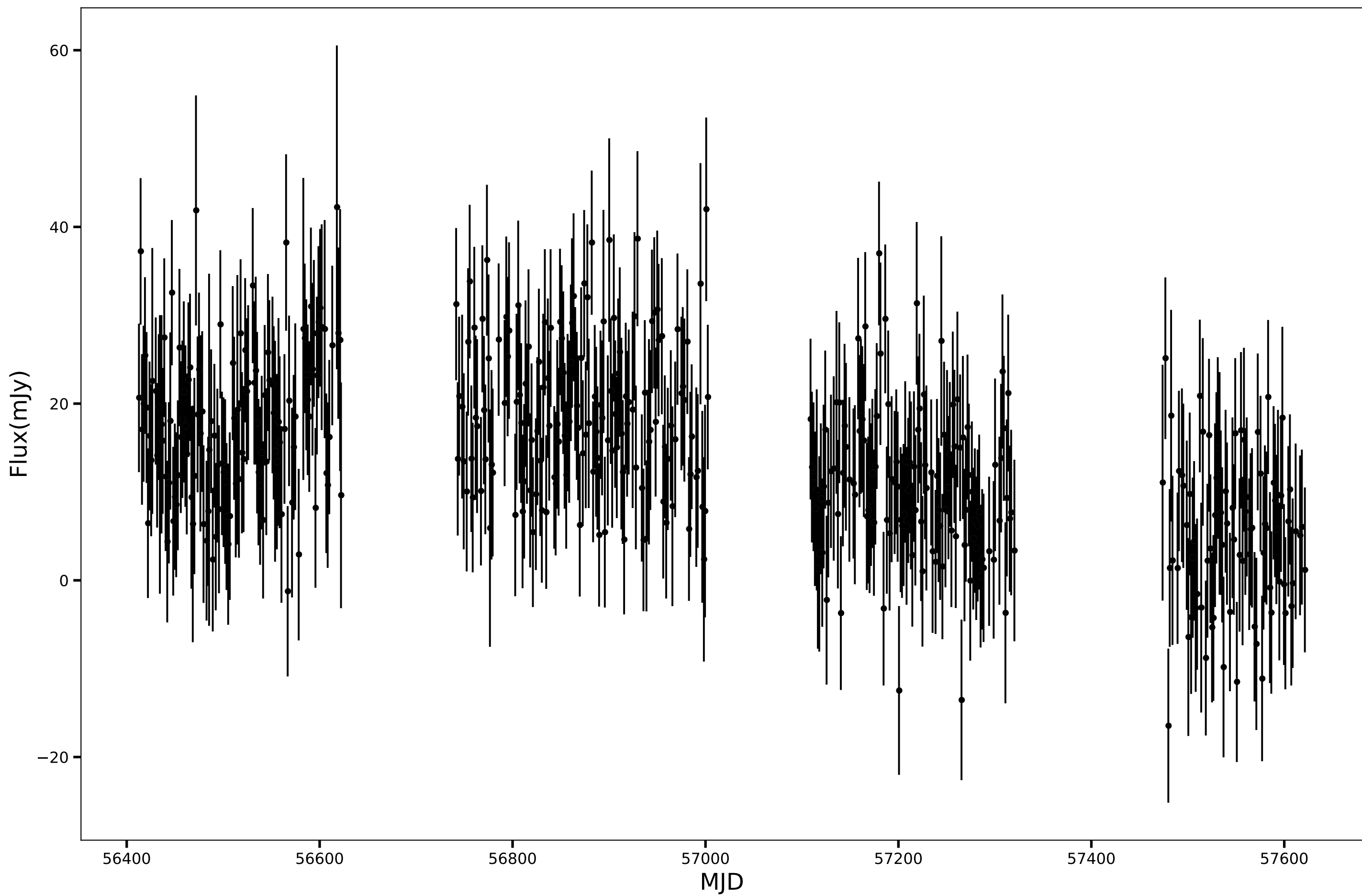
SPT-SJ234845-5847.0, RA=357.1886d, DEC=-58.7842d, mean_flux=14.20 (mJy), 150GHz
