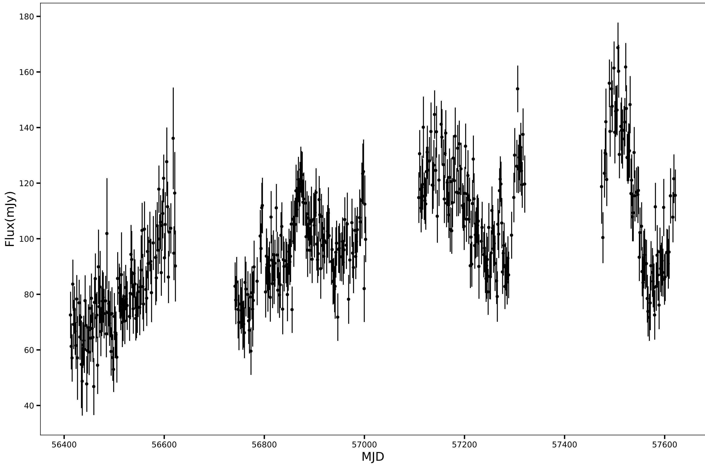
SPT-SJ234825-6049.2, RA=357.1046d, DEC=-60.8211d, mean_flux=98.77 (mJy), 150GHz
