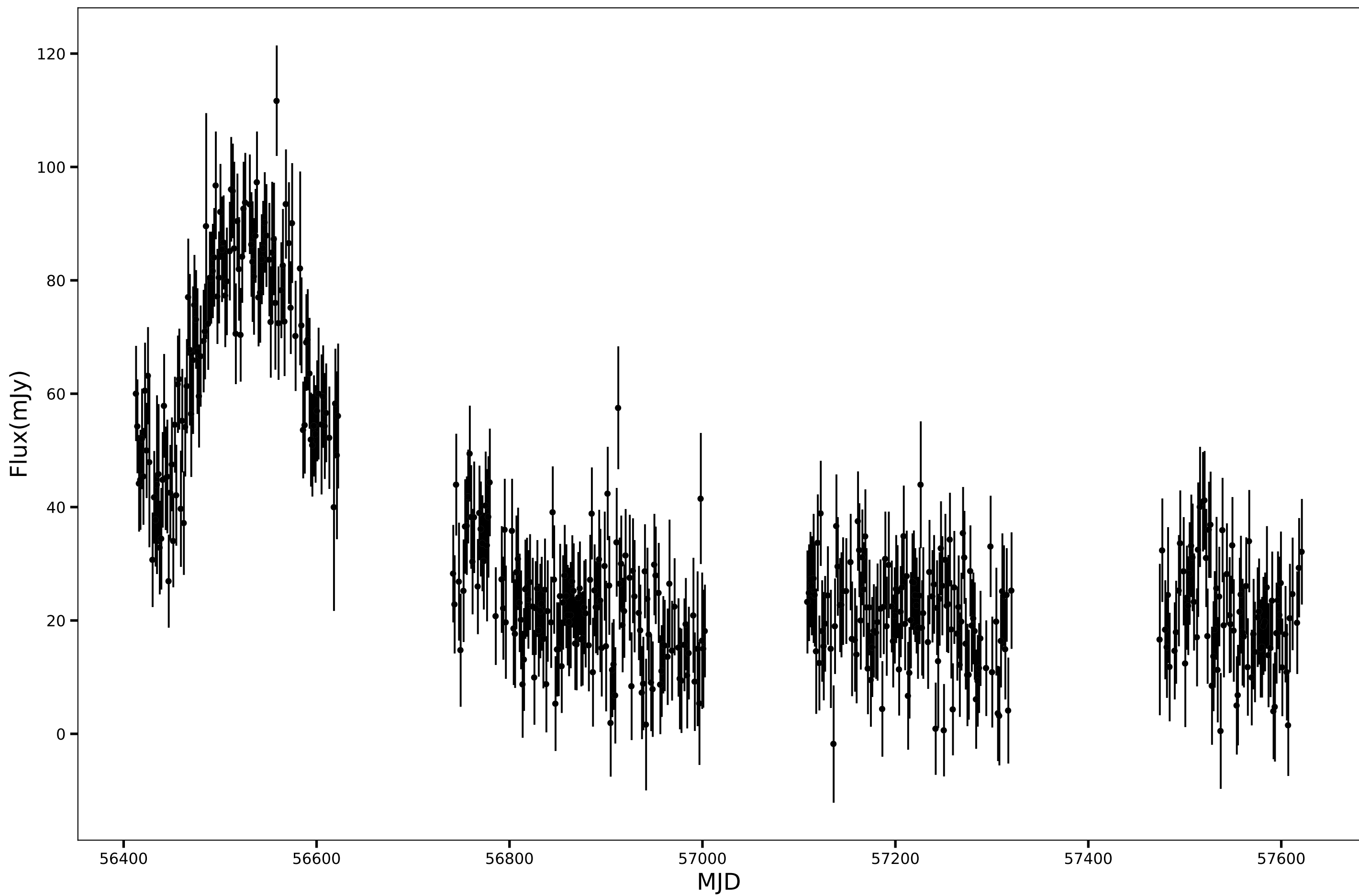
SPT-SJ234751-5915.5, RA=356.9662d, DEC=-59.2597d, mean_flux=33.63 (mJy), 150GHz
