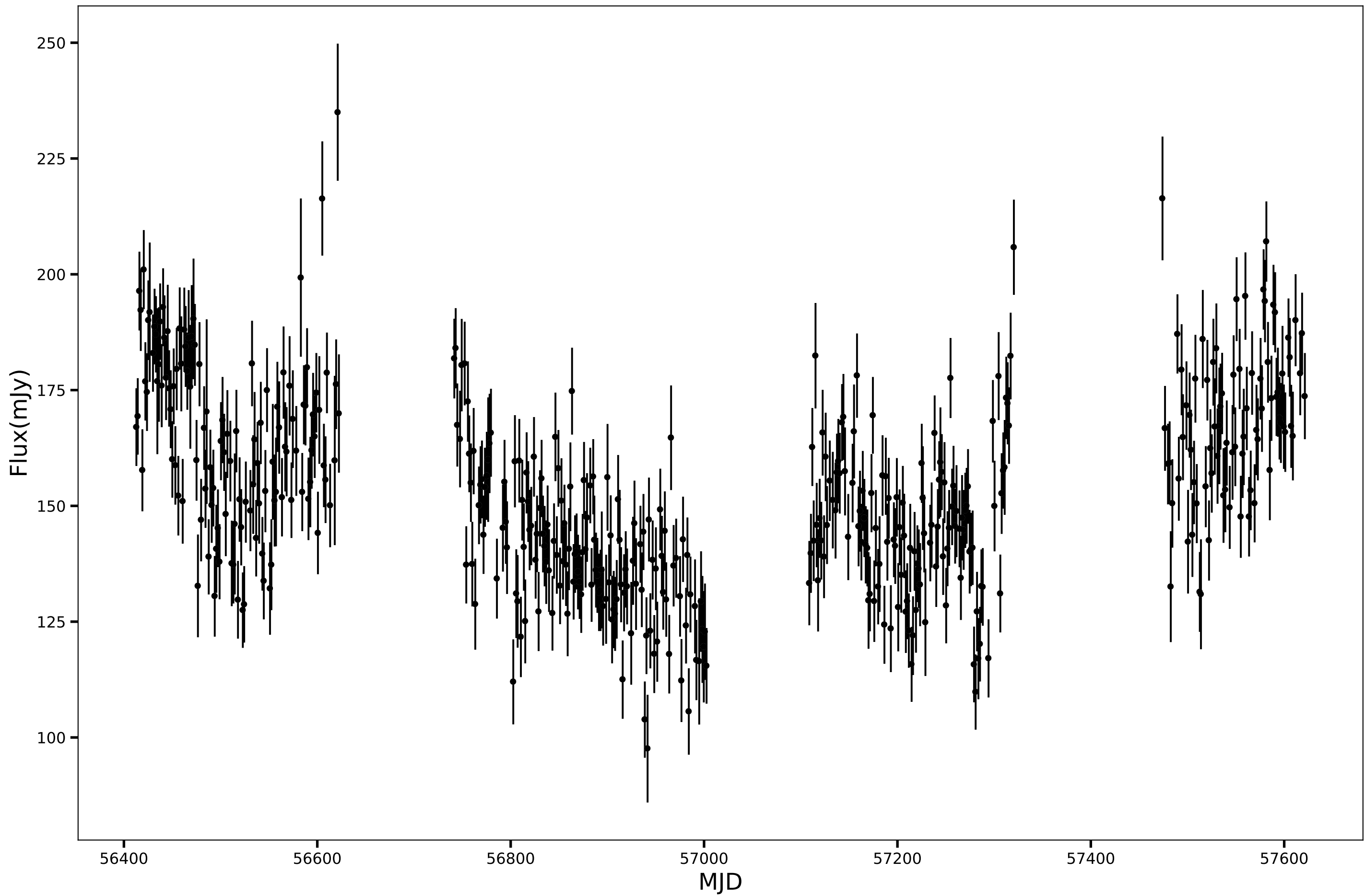
SPT-SJ234743-4946.4, RA=356.9326d, DEC=-49.7745d, mean_flux=153.37 (mJy), 150GHz
