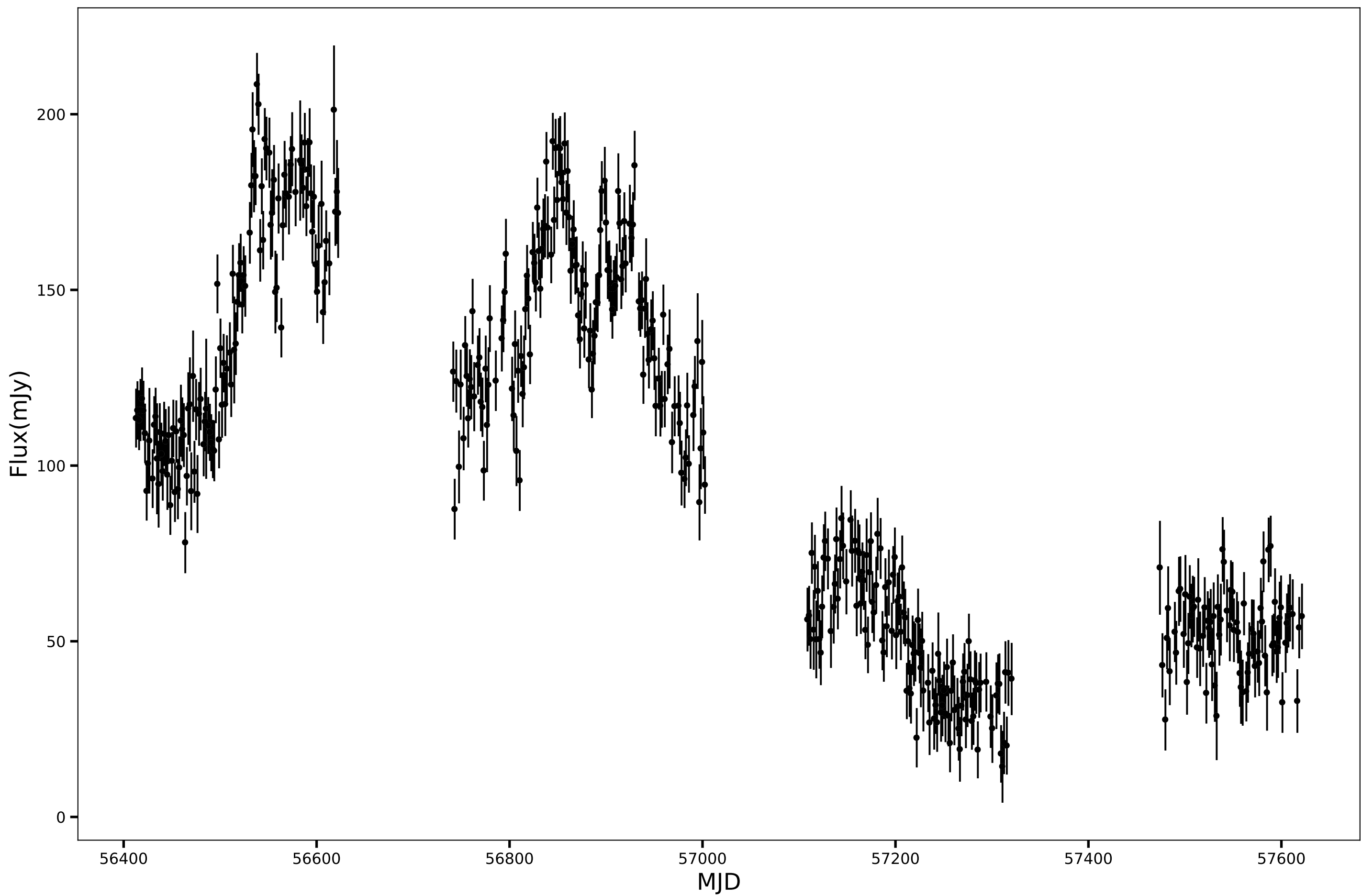
SPT-SJ234327-5626.2, RA=355.8628d, DEC=-56.4373d, mean_flux=101.78 (mJy), 150GHz
