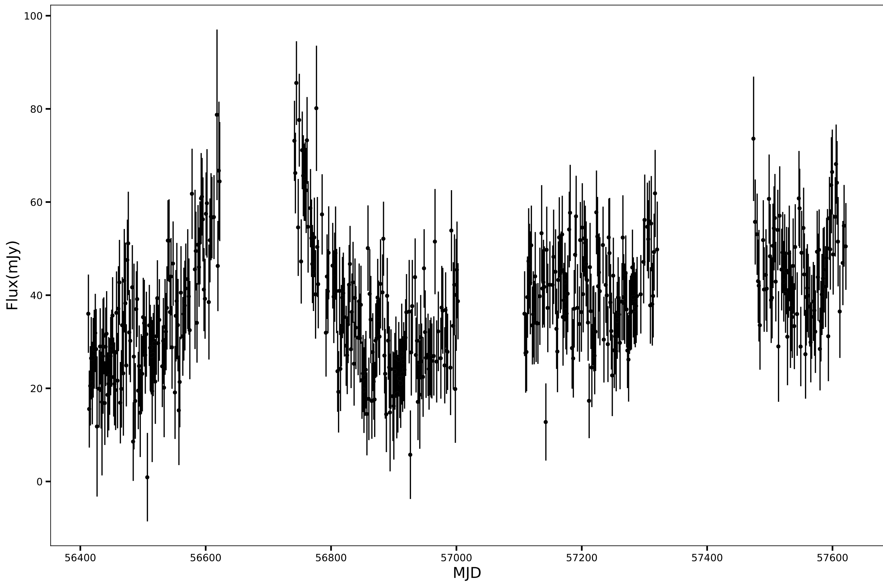
SPT-SJ234316-5709.4, RA=355.8208d, DEC=-57.1583d, mean_flux=38.23 (mJy), 150GHz
