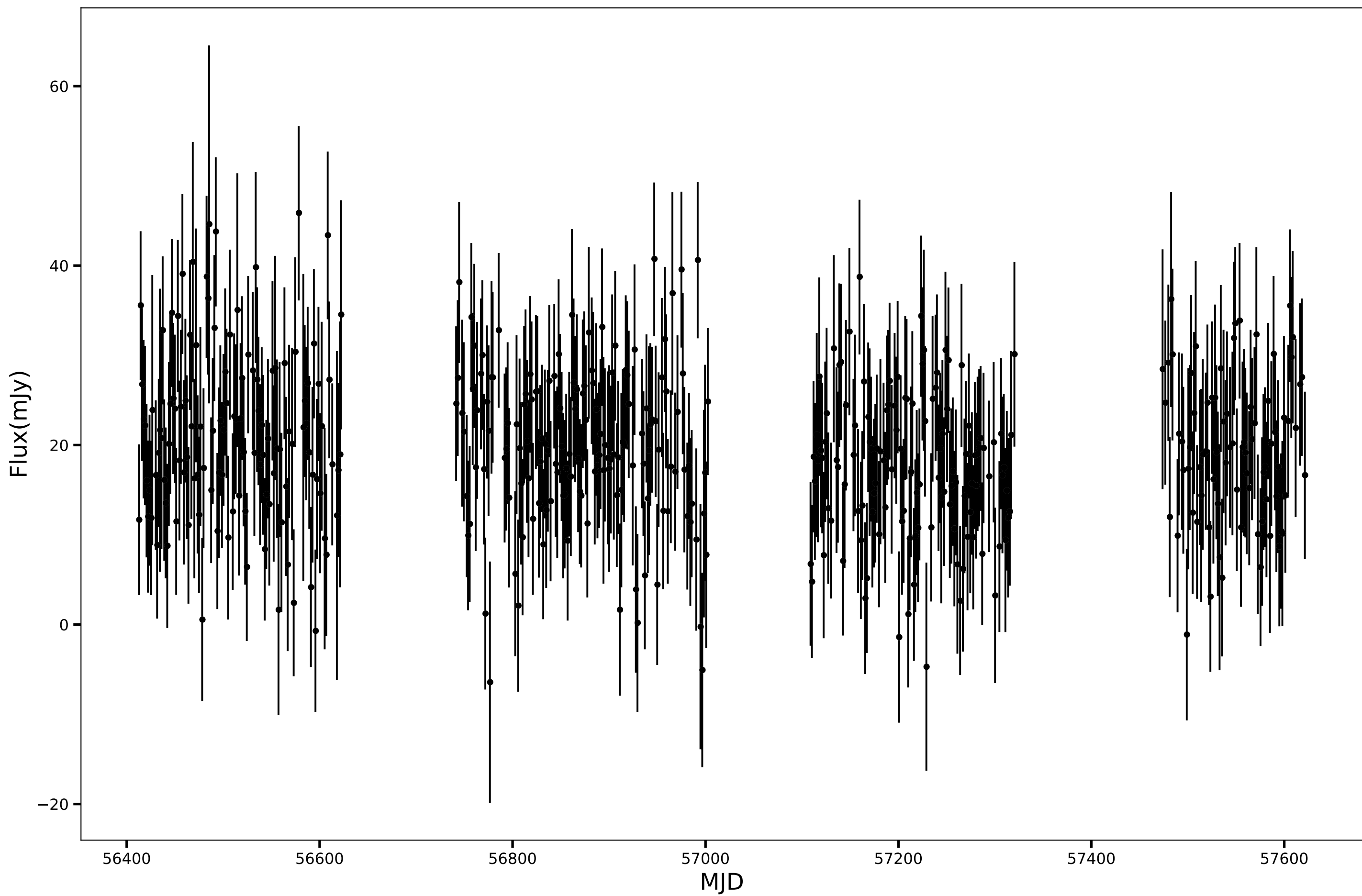
SPT-SJ234118-5816.0, RA=355.3279d, DEC=-58.2671d, mean_flux=19.58 (mJy), 150GHz
