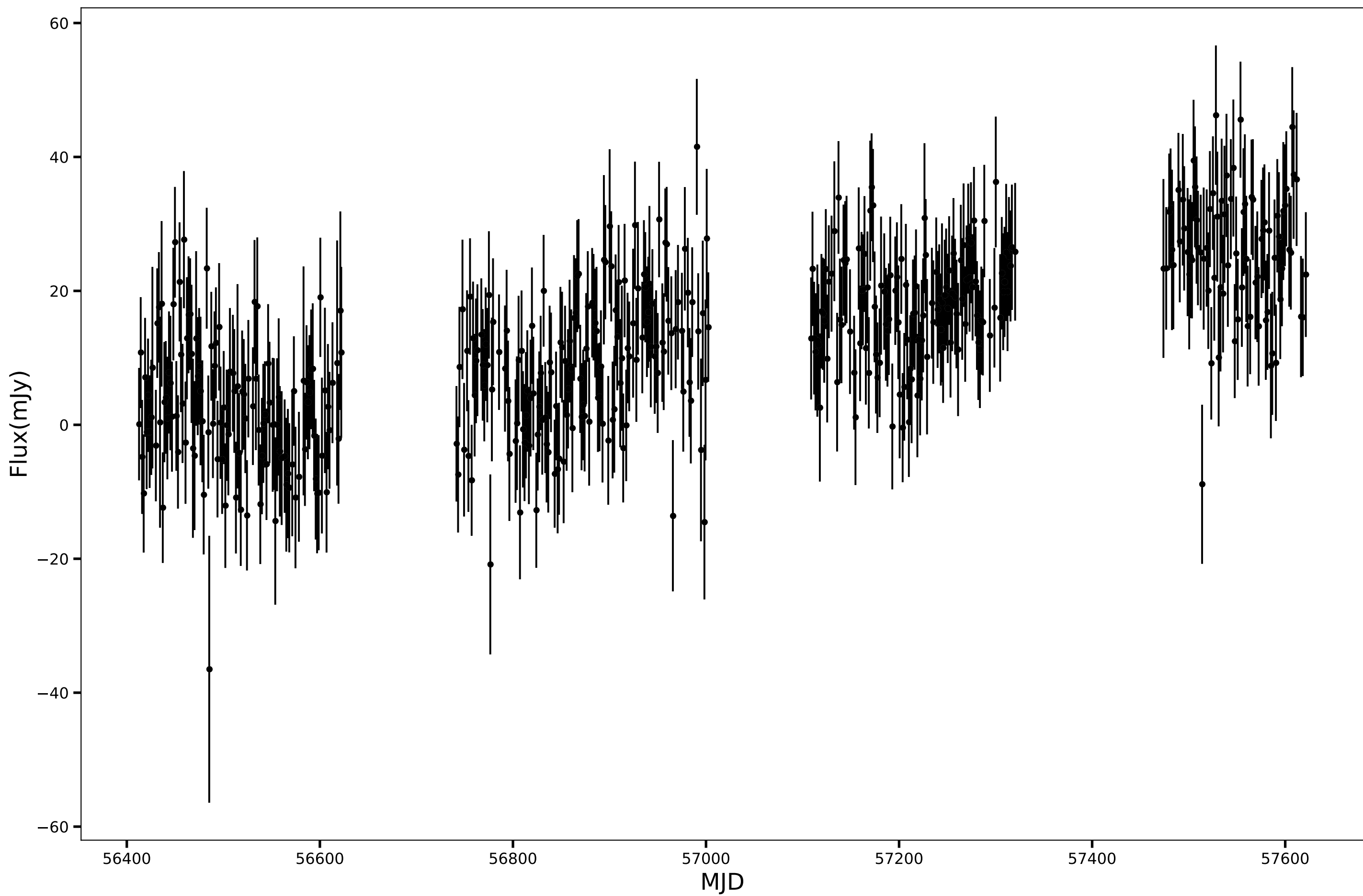
SPT-SJ233913-5523.7, RA=354.8046d, DEC=-55.3963d, mean_flux=12.48 (mJy), 150GHz
