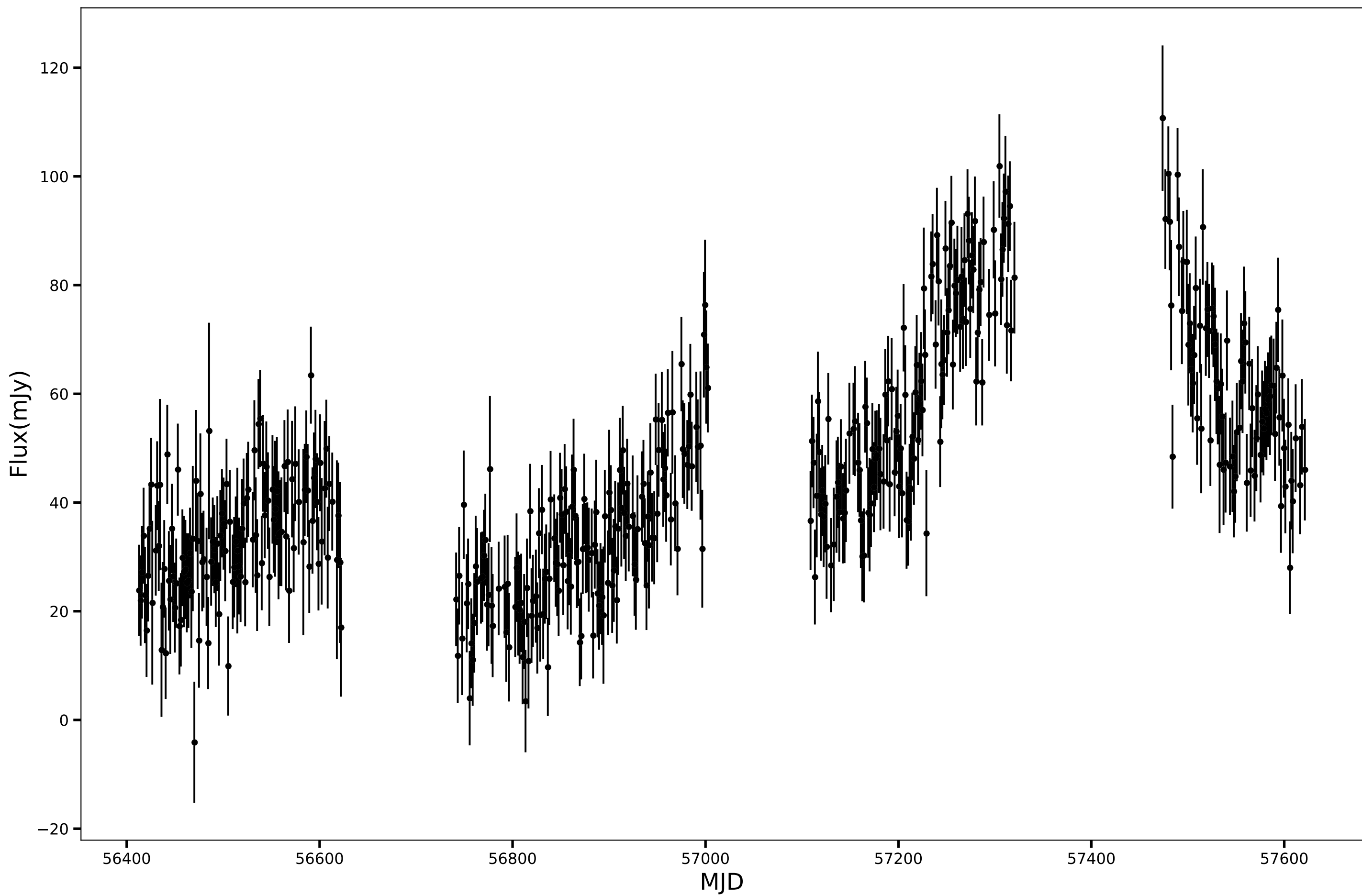
SPT-SJ233726-5901.1, RA=354.3605d, DEC=-59.0184d, mean_flux=44.97 (mJy), 150GHz
