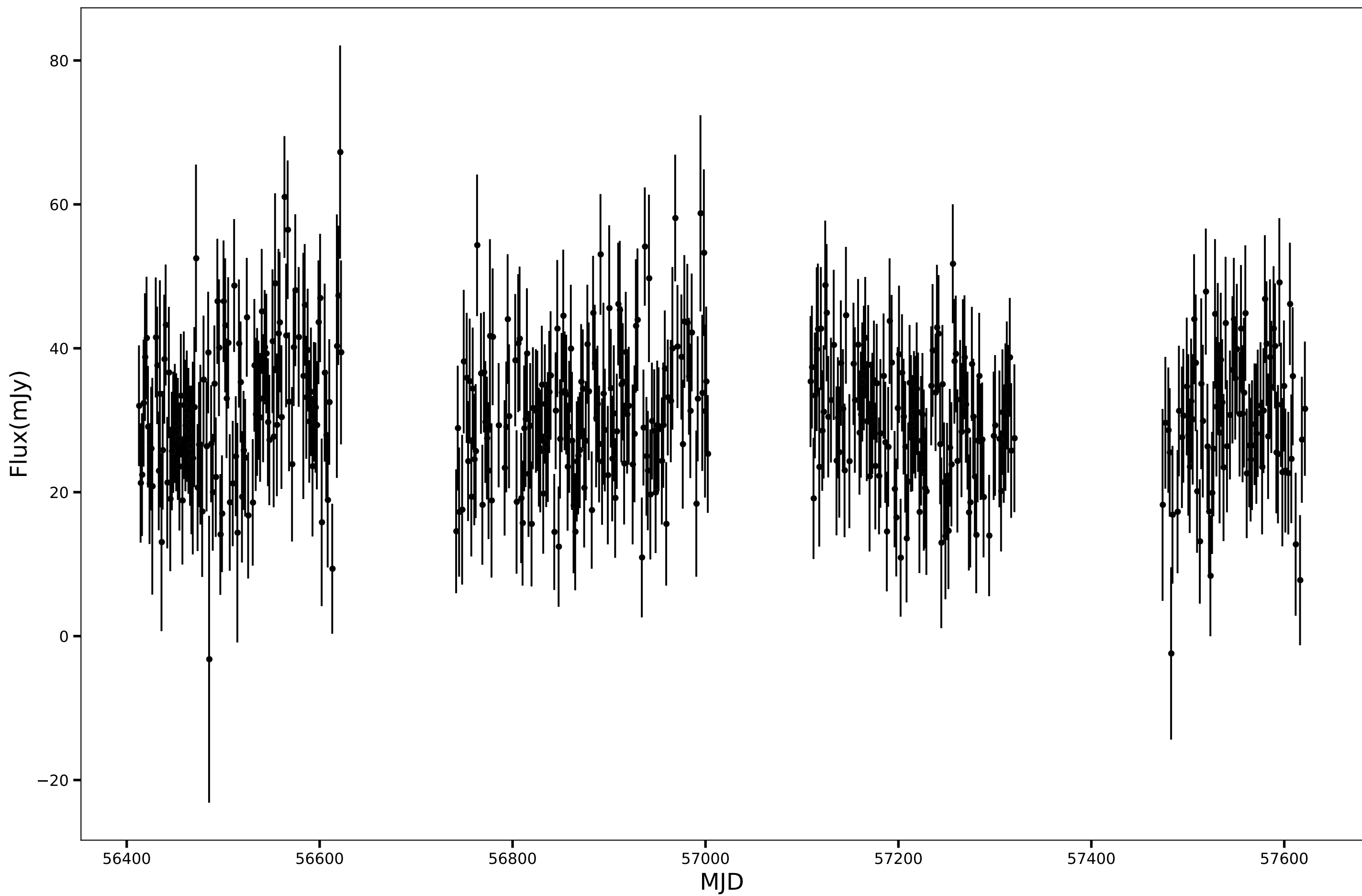
SPT-SJ233723-5216.2, RA=354.3465d, DEC=-52.2710d, mean_flux=30.85 (mJy), 150GHz
