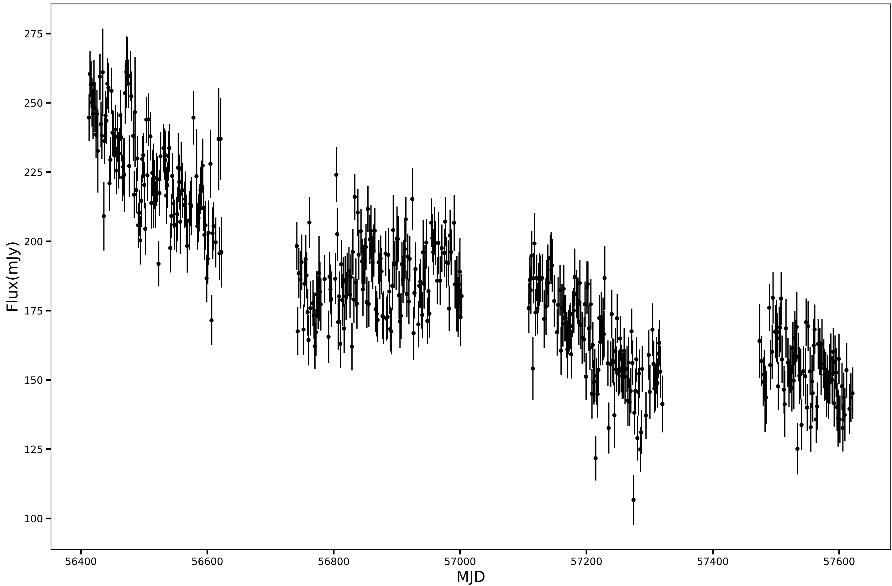
SPT-SJ233444-5251.2, RA=353.6866d, DEC=-52.8546d, mean_flux=185.31 (mJy), 150GHz
