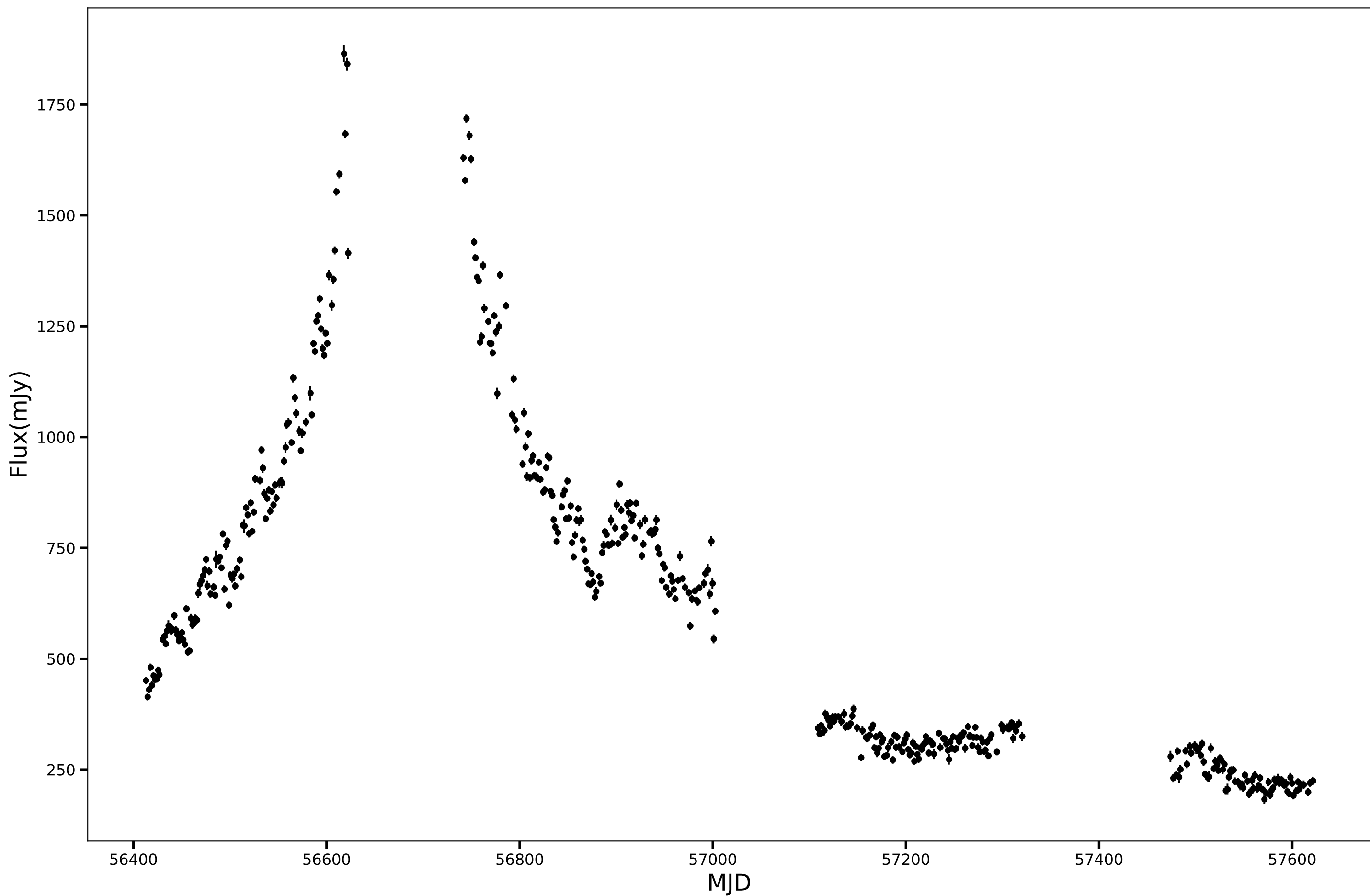
SPT-SJ232920-4955.6, RA=352.3370d, DEC=-49.9276d, mean_flux=614.26 (mJy), 150GHz
