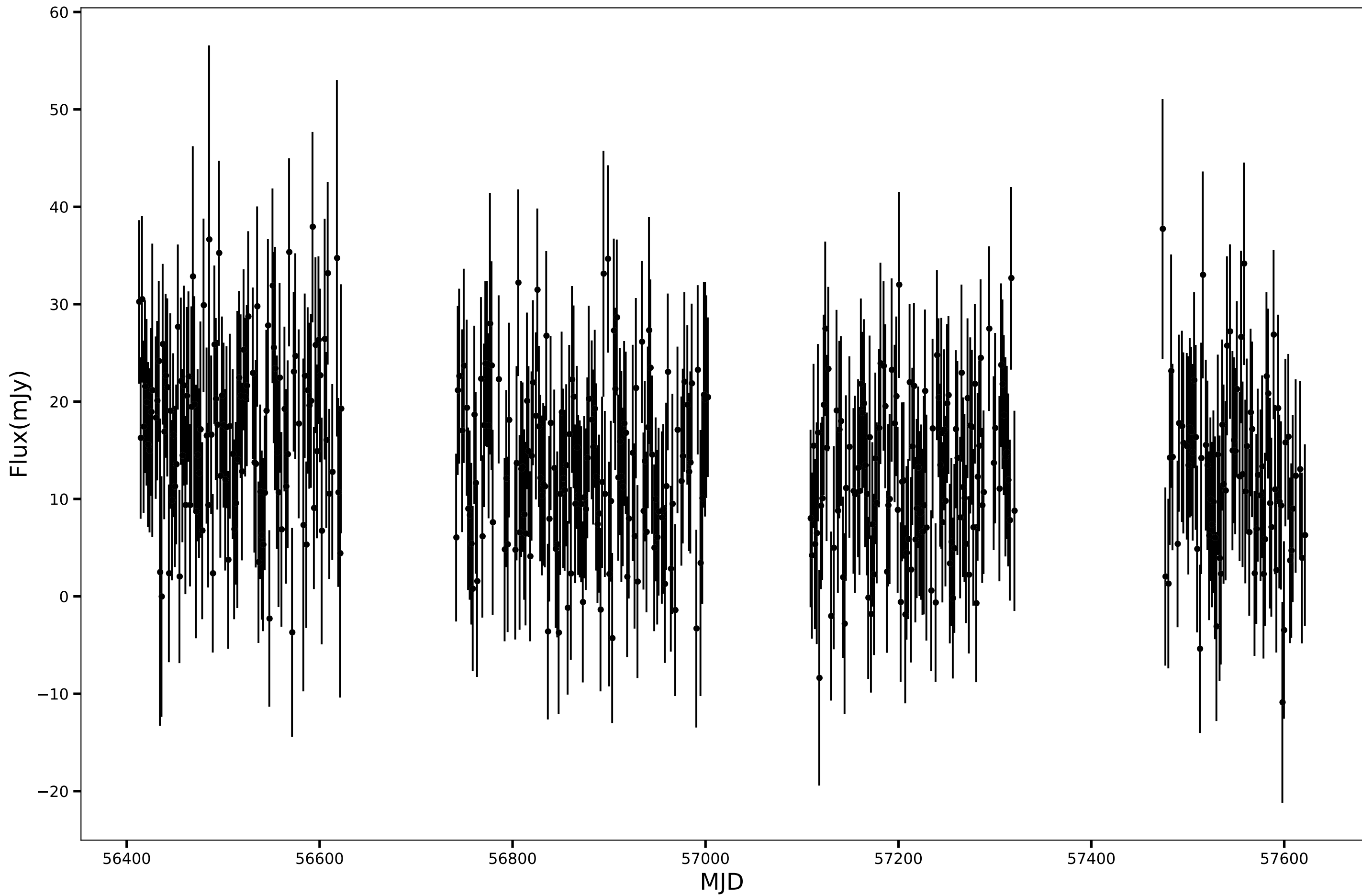
SPT-SJ232510-5656.4, RA=351.2957d, DEC=-56.9409d, mean_flux=14.02 (mJy), 150GHz
