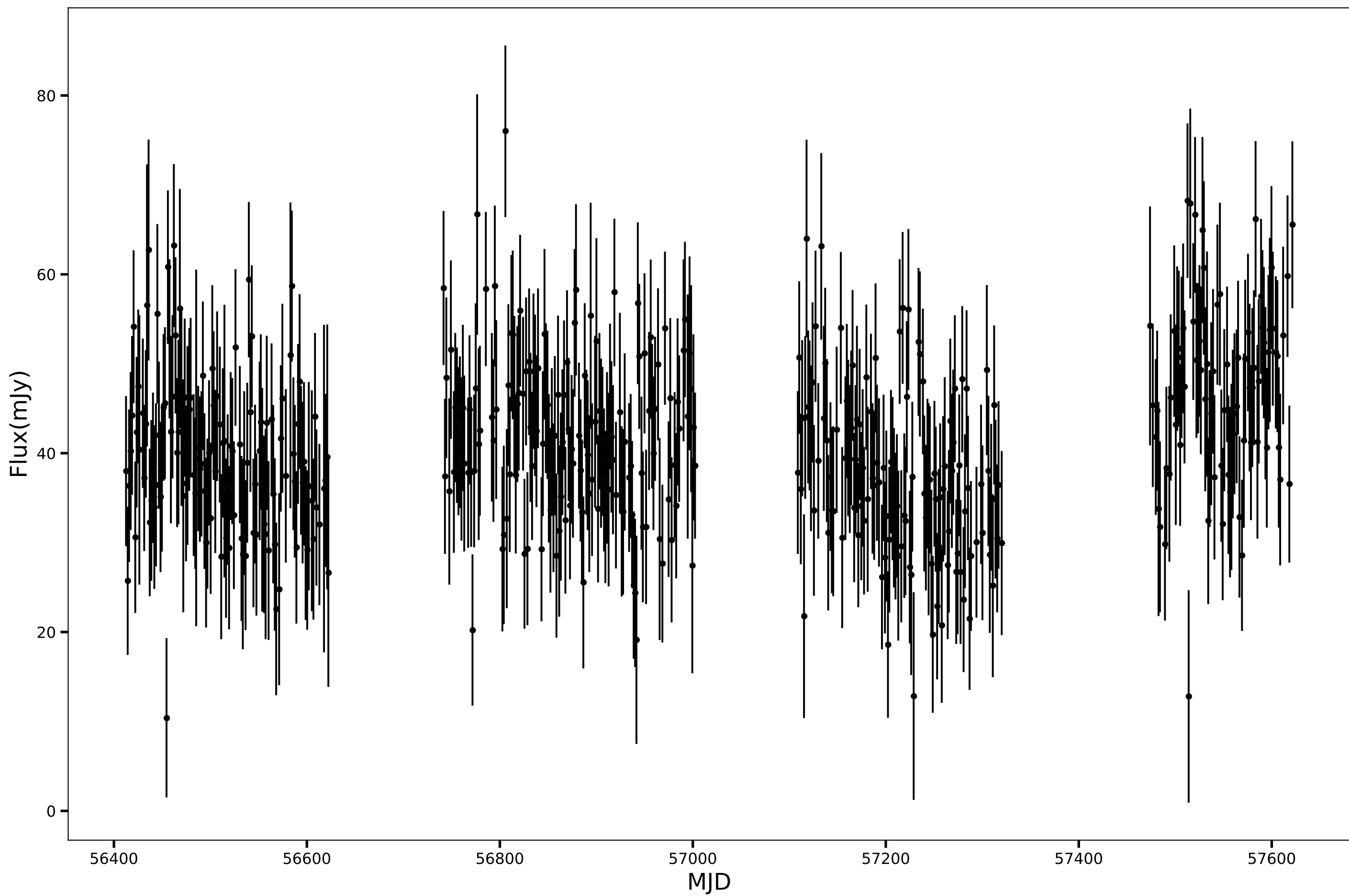
SPT-SJ232142-6438.1, RA=350.4284d, DEC=-64.6362d, mean_flux=41.06 (mJy), 150GHz
