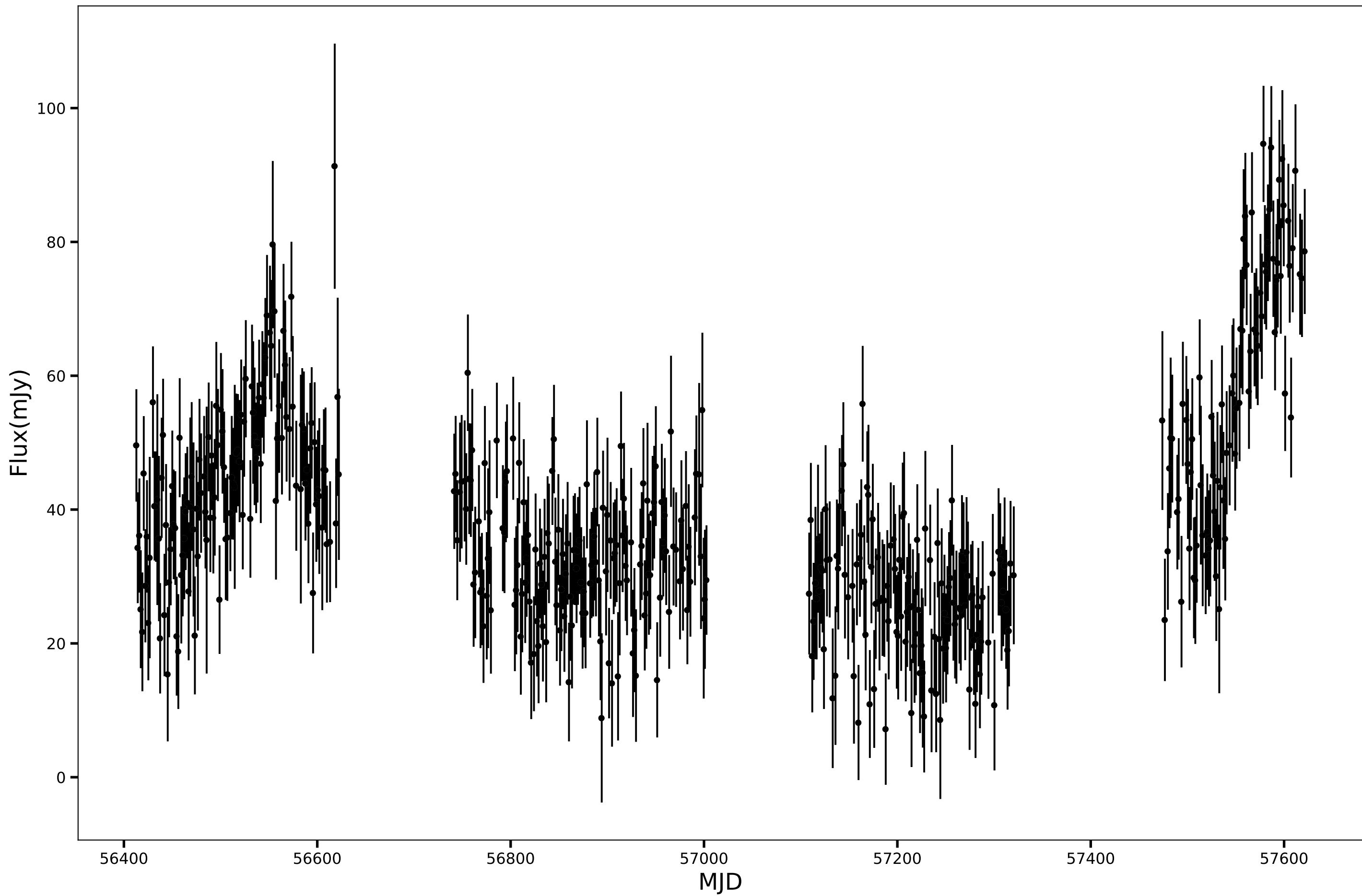
SPT-SJ232100-5402.5, RA=350.2506d, DEC=-54.0424d, mean_flux=38.70 (mJy), 150GHz
