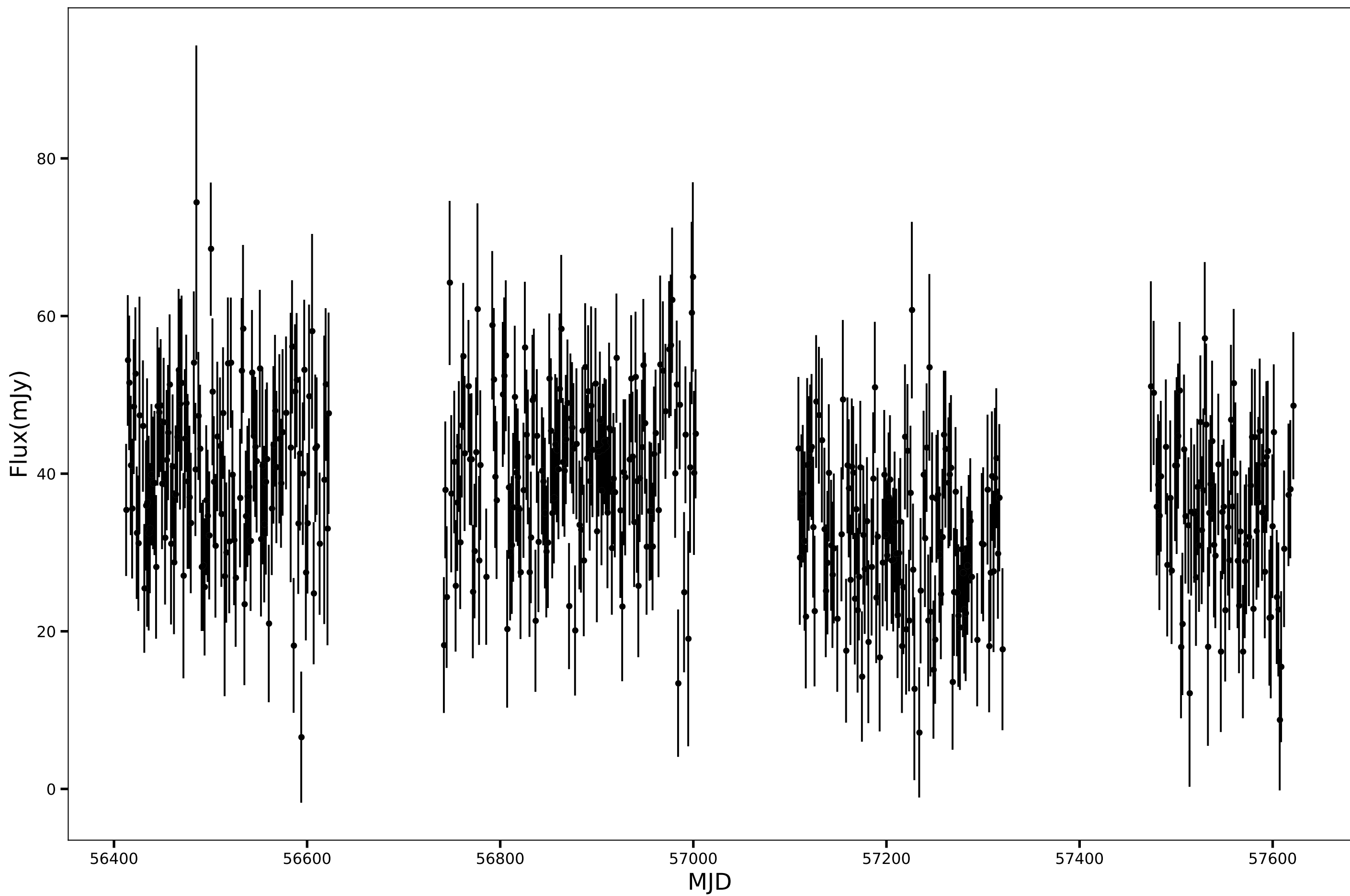
SPT-SJ232047-5309.7, RA=350.1998d, DEC=-53.1617d, mean_flux=37.37 (mJy), 150GHz
