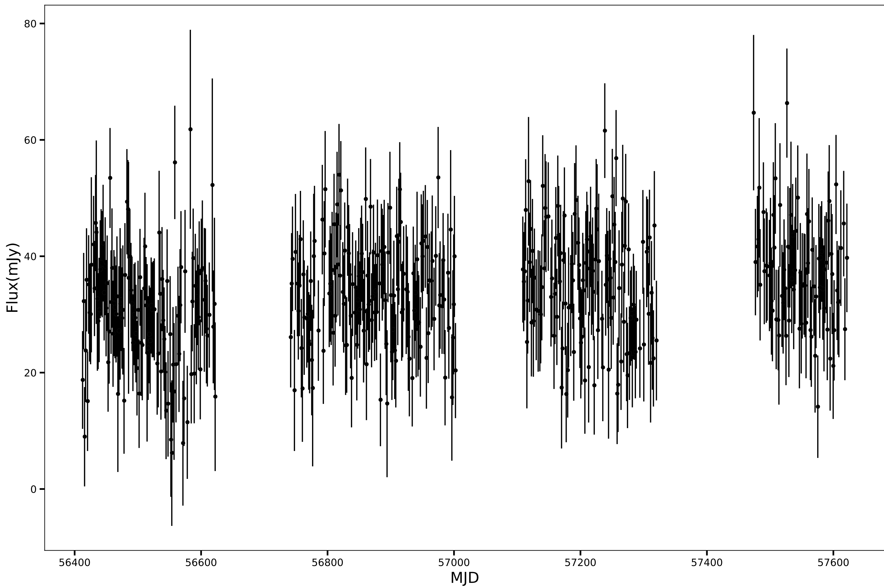
SPT-SJ231916-5331.8, RA=349.8185d, DEC=-53.5308d, mean_flux=33.68 (mJy), 150GHz
