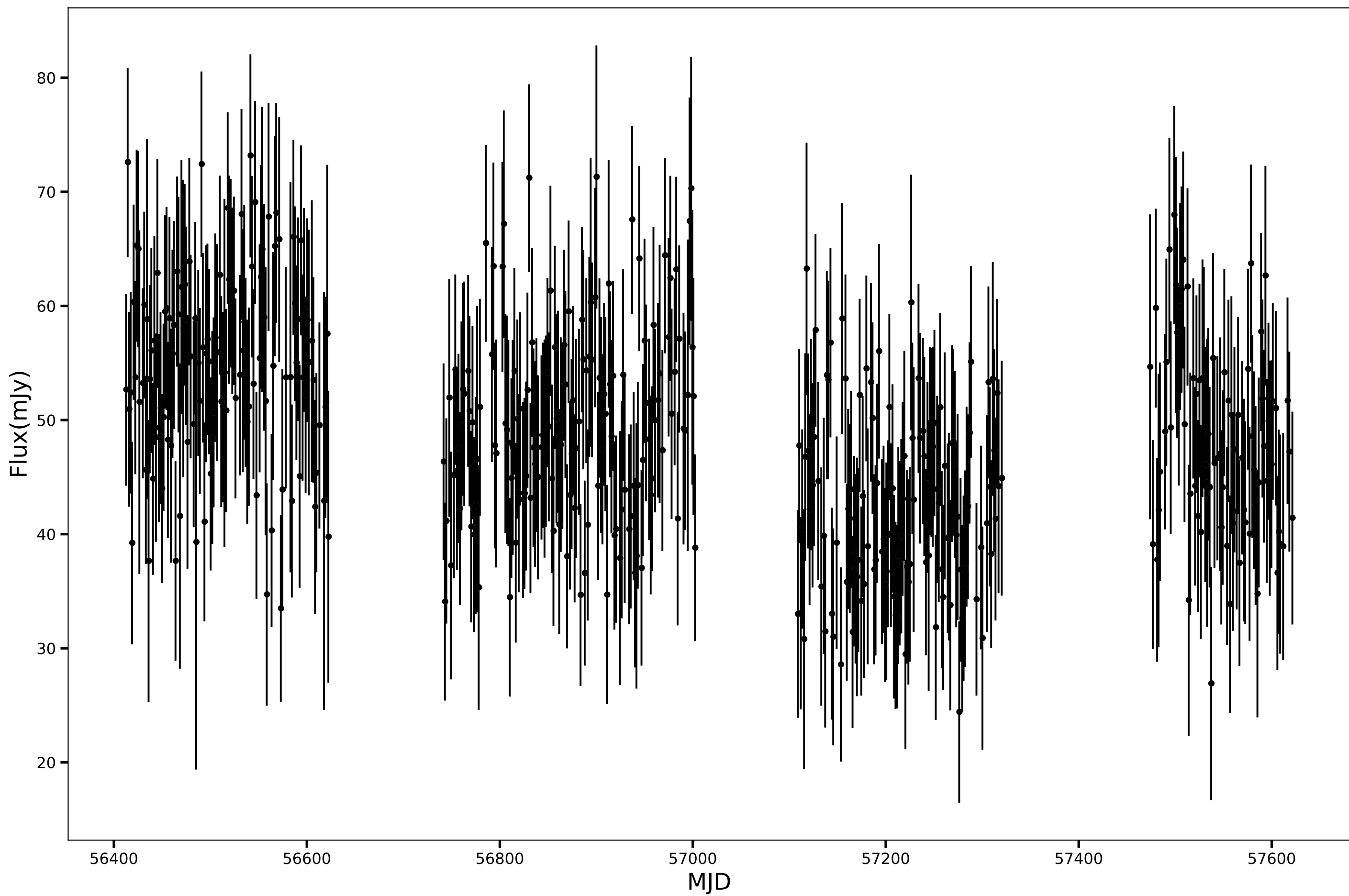
SPT-SJ231716-6215.3, RA=349.3194d, DEC=-62.2563d, mean_flux=48.80 (mJy), 150GHz
