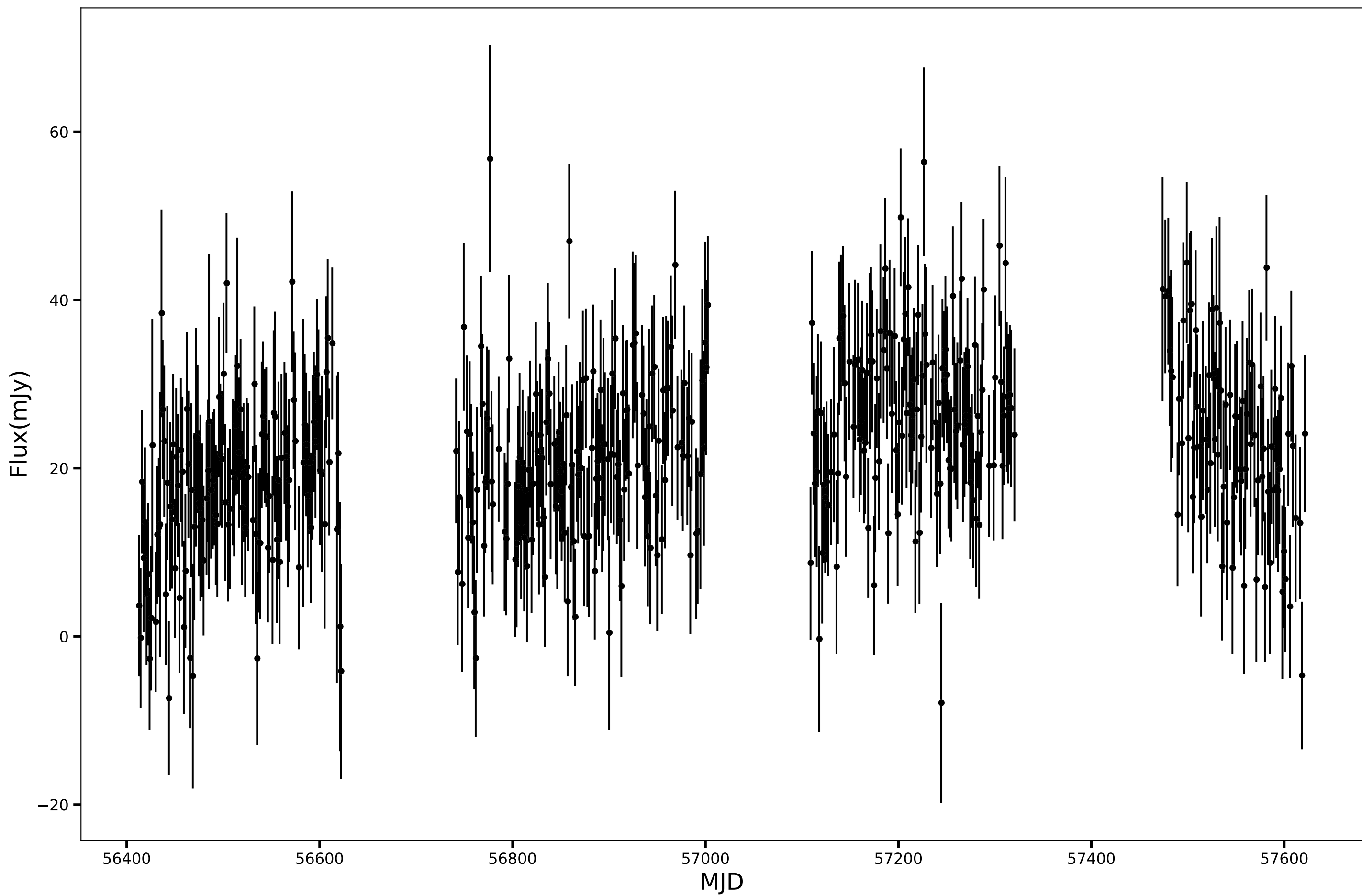
SPT-SJ231653-5507.8, RA=349.2224d, DEC=-55.1311d, mean_flux=21.87 (mJy), 150GHz
