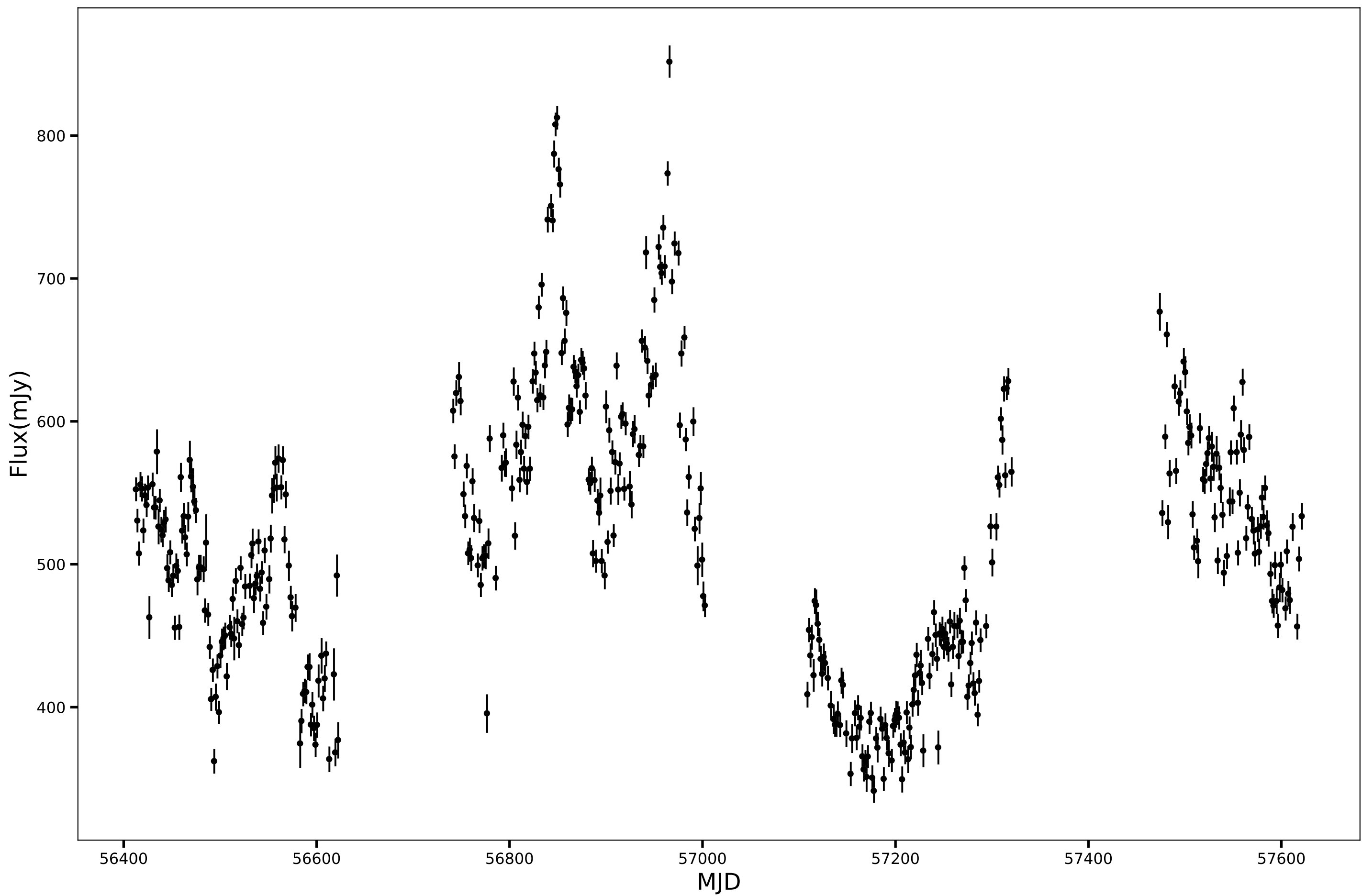
SPT-SJ231545-5018.6, RA=348.9388d, DEC=-50.3106d, mean_flux=516.19 (mJy), 150GHz
