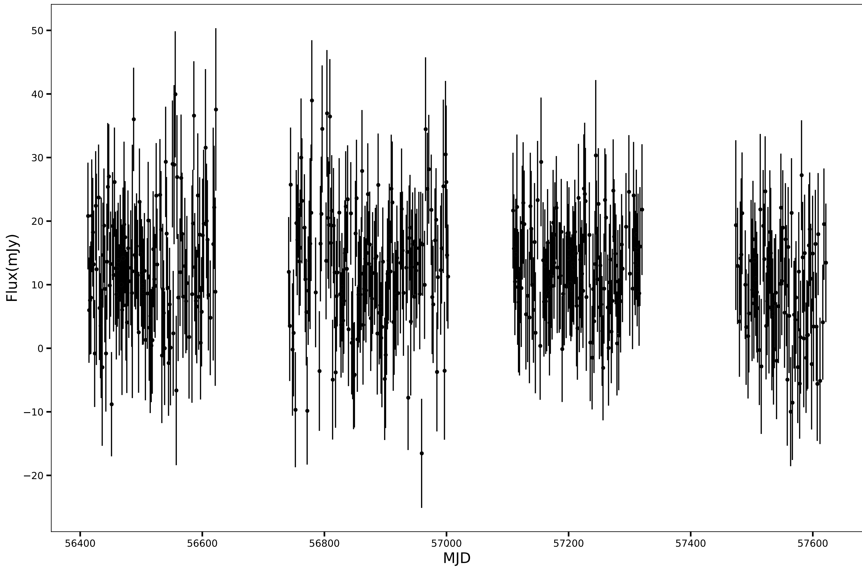
SPT-SJ231109-5624.7, RA=347.7895d, DEC=-56.4123d, mean_flux=12.08 (mJy), 150GHz
