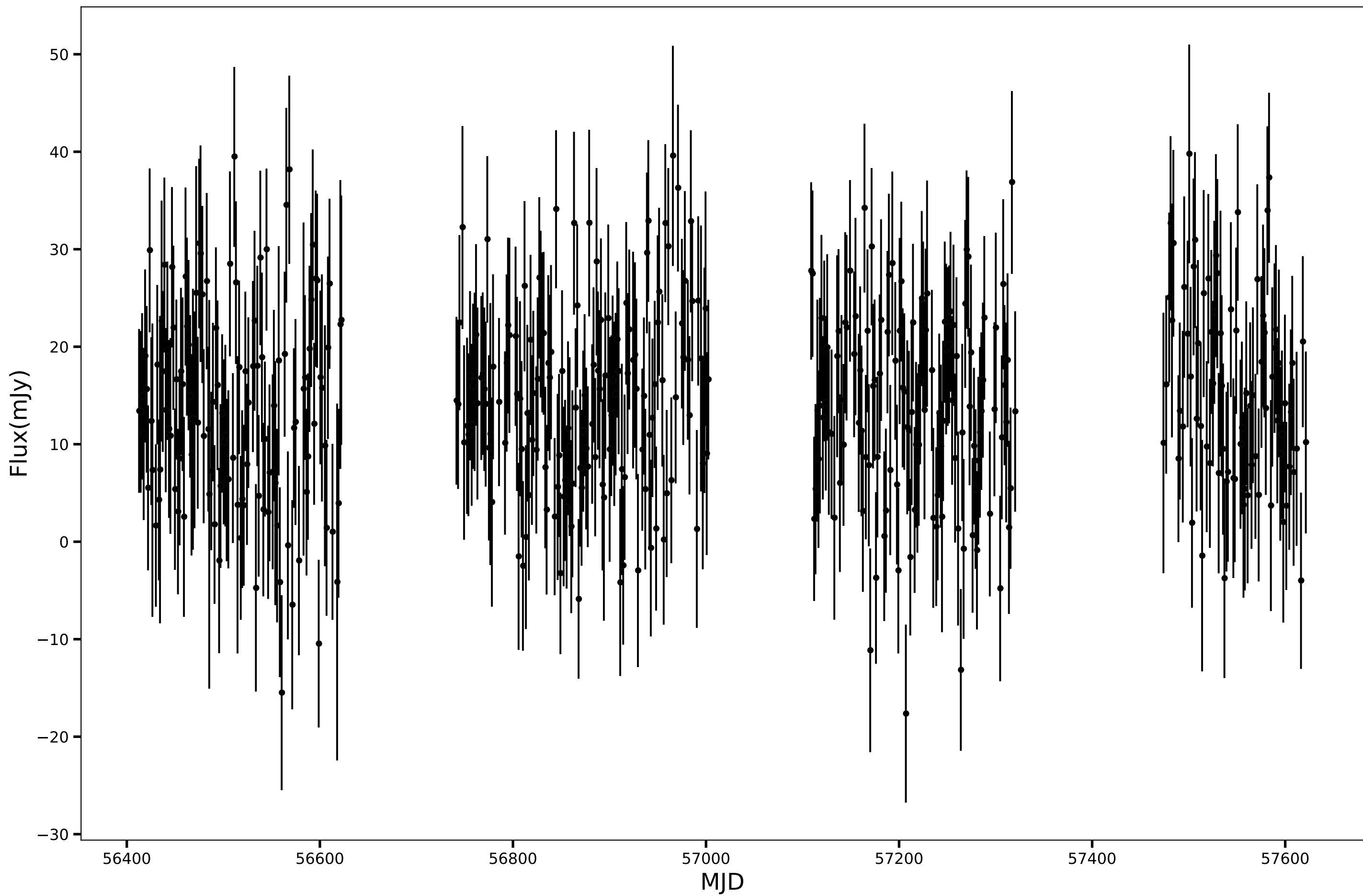
SPT-SJ225647-5158.7, RA=344.1983d, DEC=-51.9785d, mean_flux=14.30 (mJy), 150GHz
