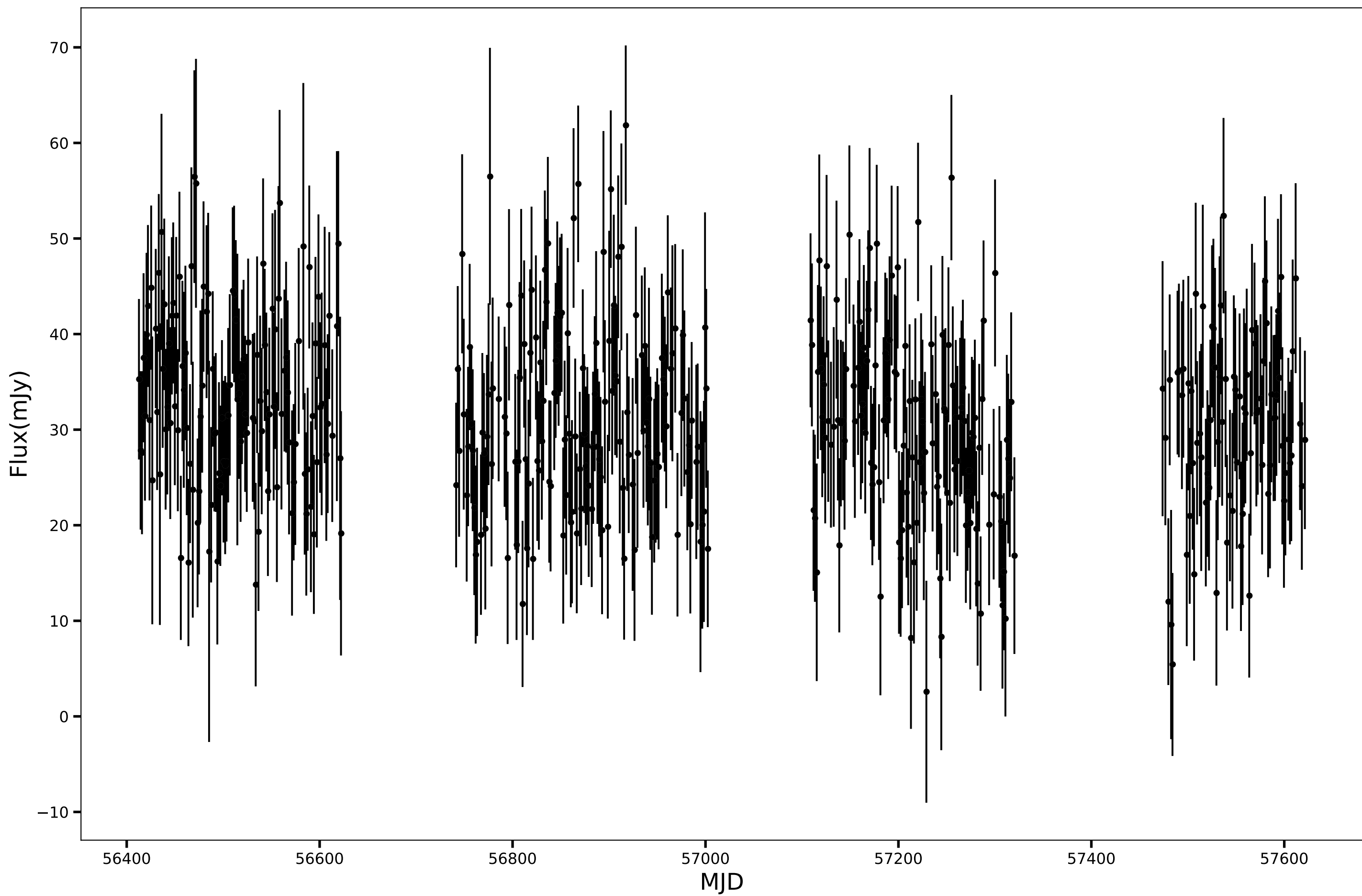
SPT-SJ225550-5245.7, RA=343.9612d, DEC=-52.7621d, mean_flux=31.30 (mJy), 150GHz
