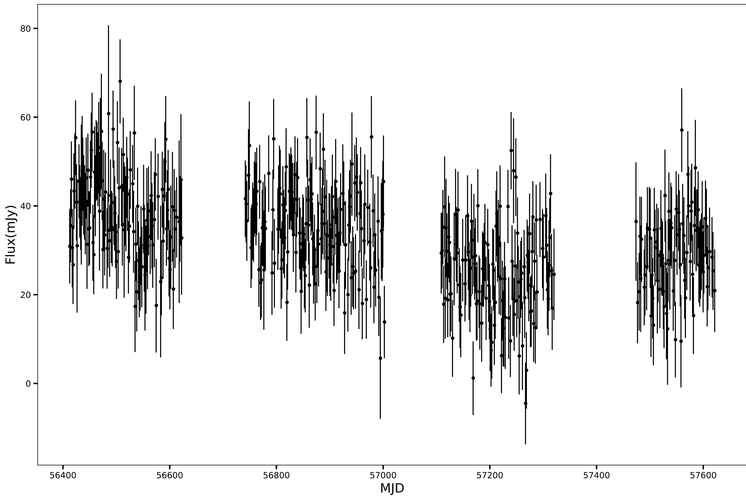
SPT-SJ225136-5453.0, RA=342.9017d, DEC=-54.8844d, mean_flux=32.31 (mJy), 150GHz
