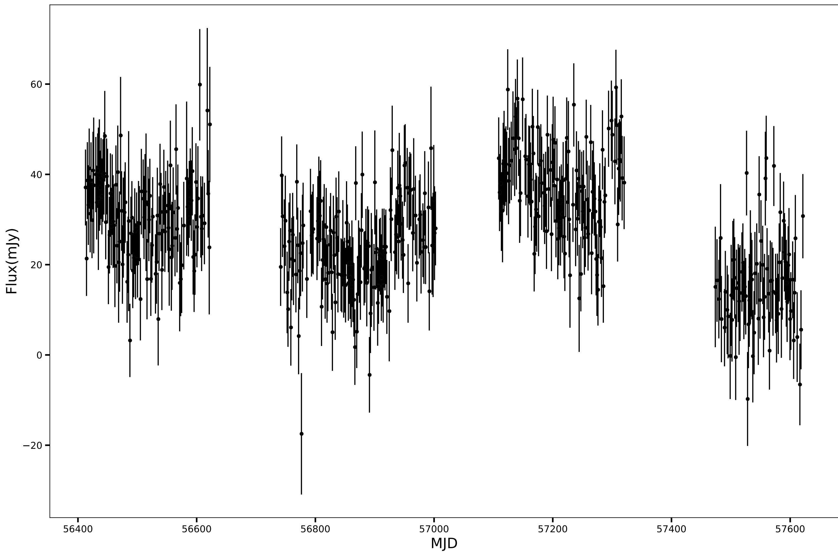
SPT-SJ224836-5933.9, RA=342.1518d, DEC=-59.5654d, mean_flux=27.49 (mJy), 150GHz
