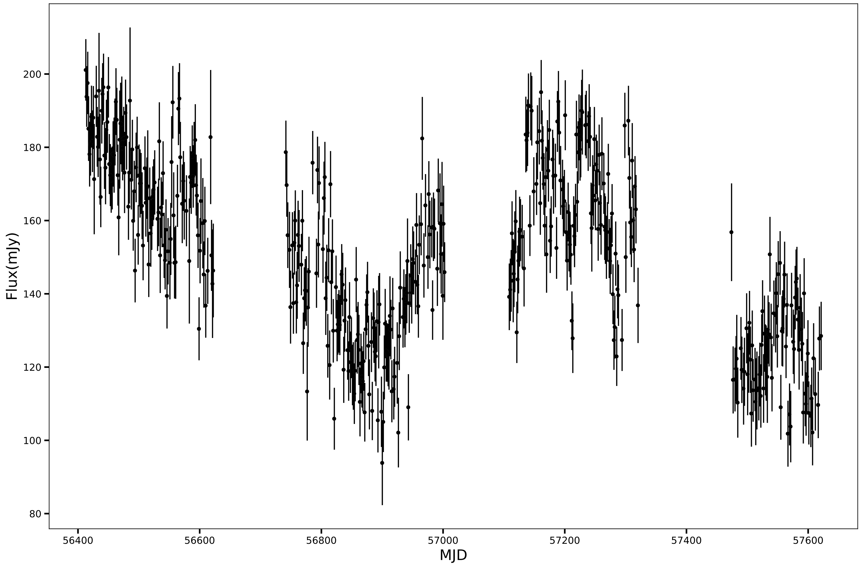
SPT-SJ224615-5607.7, RA=341.5663d, DEC=-56.1287d, mean_flux=150.88 (mJy), 150GHz
