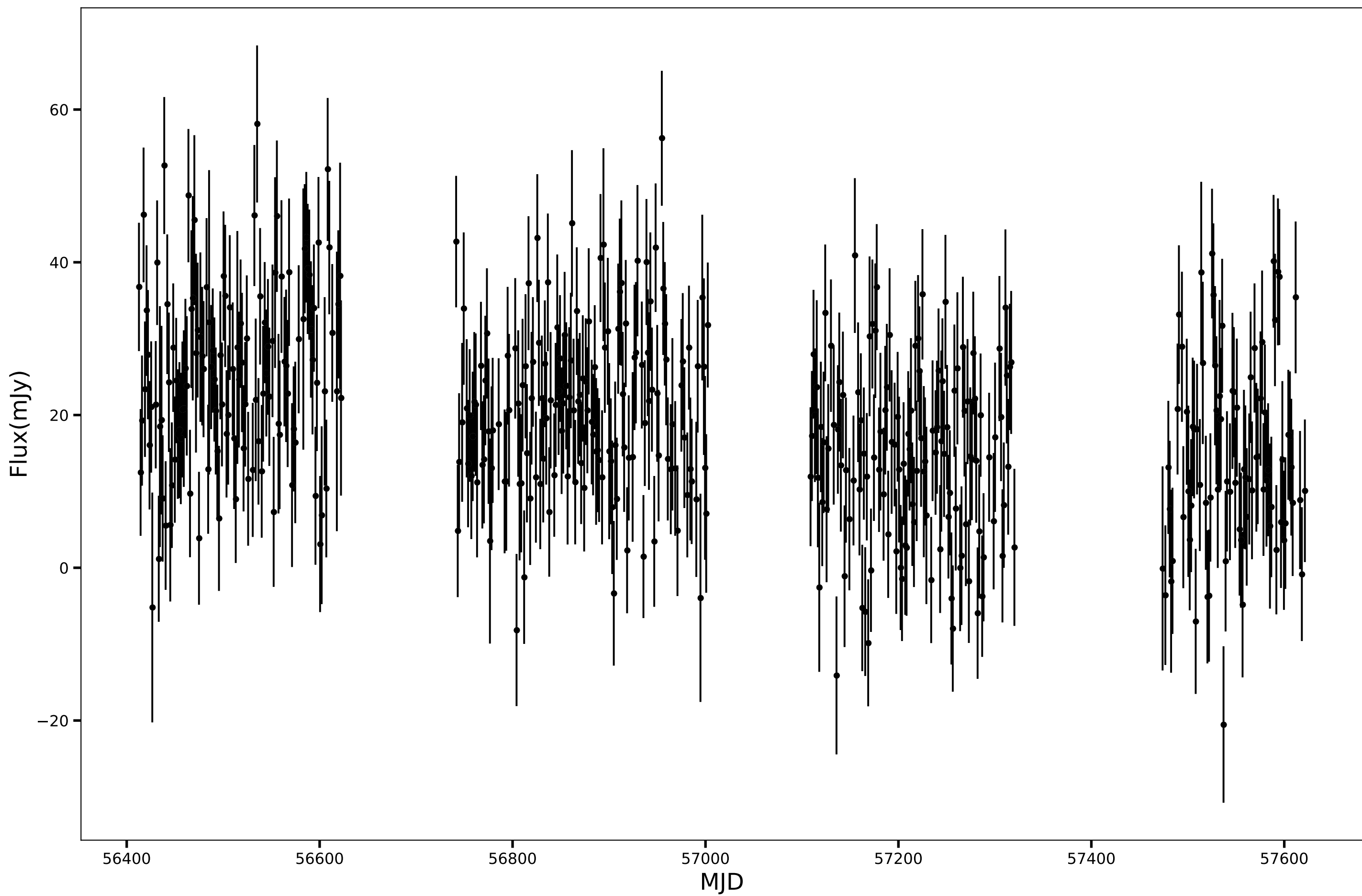
SPT-SJ224500-4931.8, RA=341.2518d, DEC=-49.5302d, mean_flux=19.28 (mJy), 150GHz
