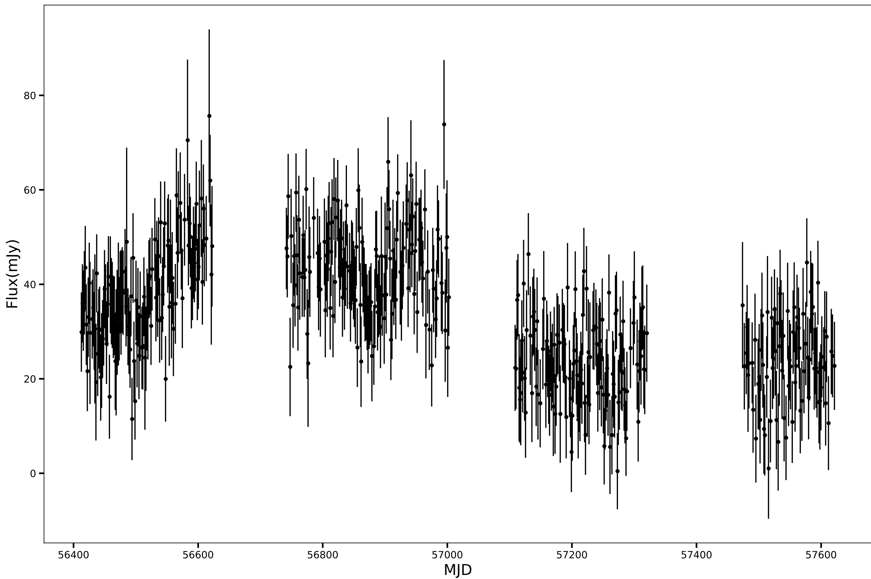
SPT-SJ224353-5656.3, RA=340.9739d, DEC=-56.9386d, mean_flux=33.33 (mJy), 150GHz
