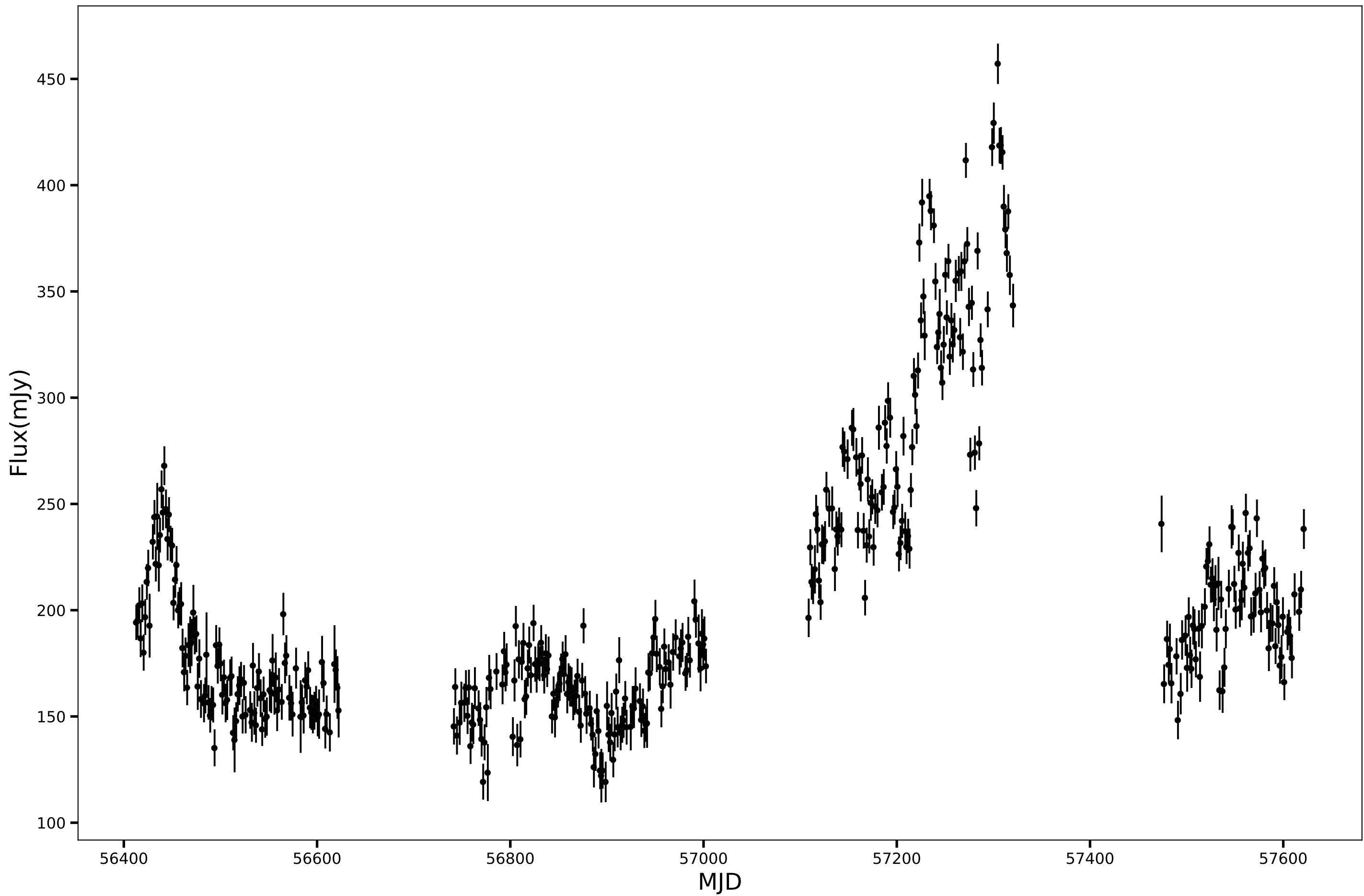
SPT-SJ224306-6250.9, RA=340.7788d, DEC=-62.8497d, mean_flux=207.12 (mJy), 150GHz
