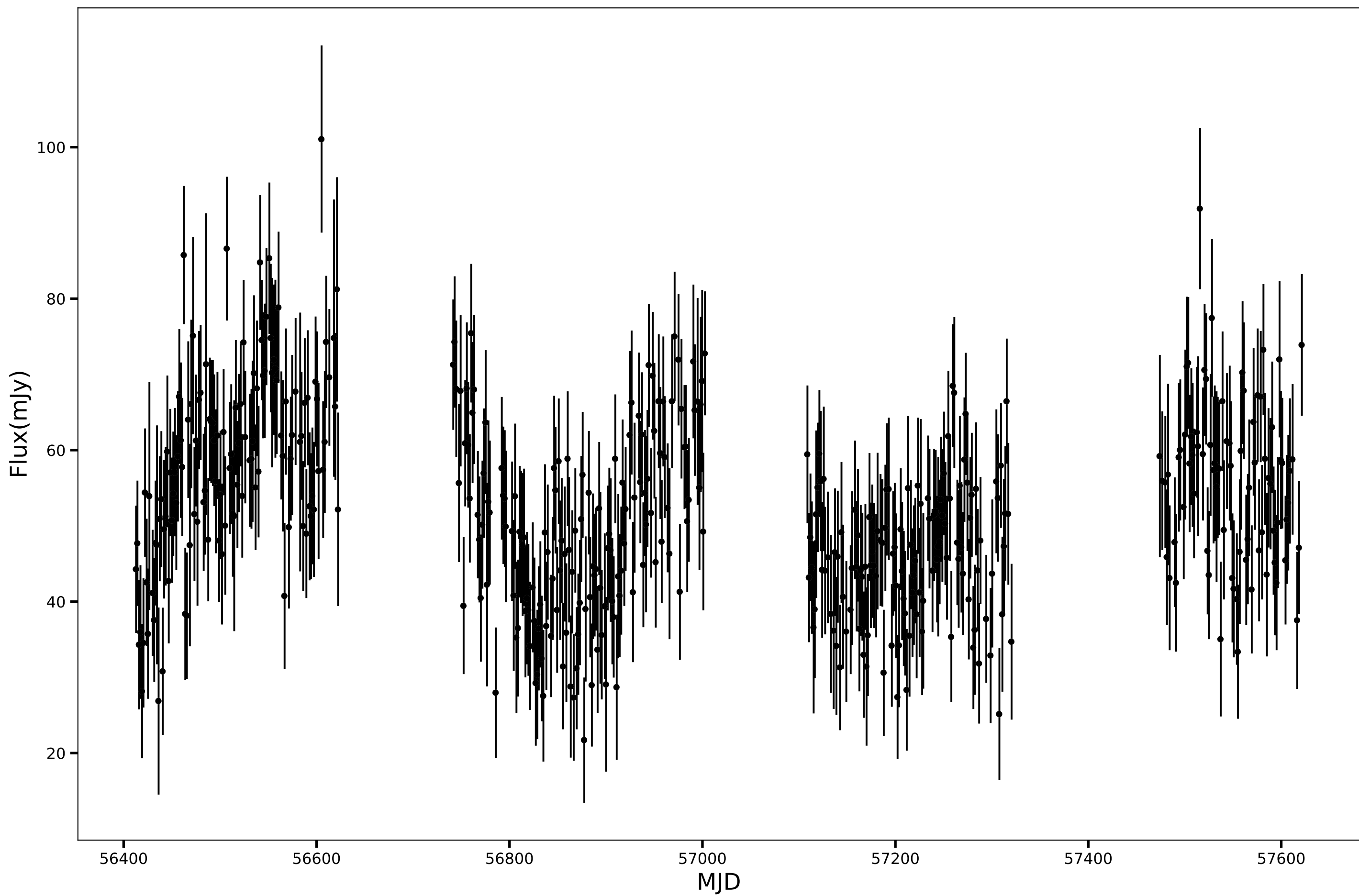
SPT-SJ224223-6044.3, RA=340.5986d, DEC=-60.7398d, mean_flux=52.20 (mJy), 150GHz
