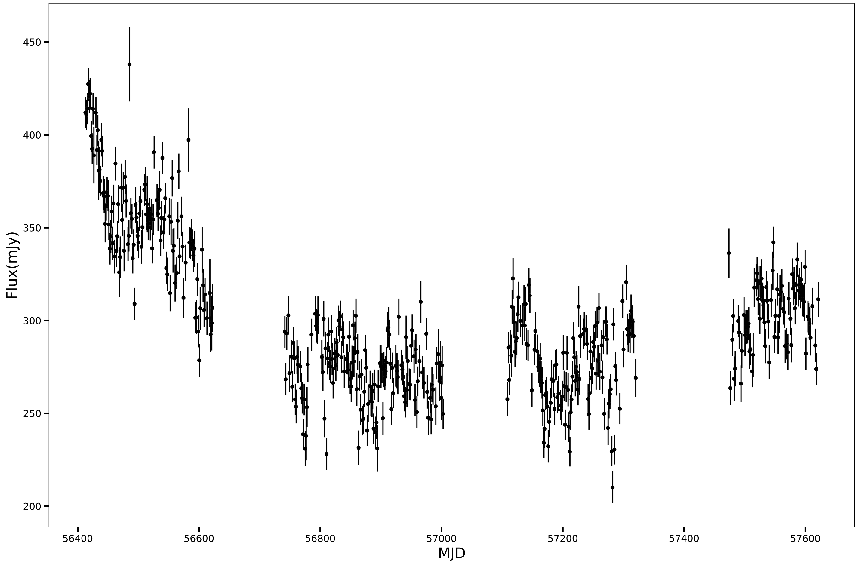
SPT-SJ223911-5701.0, RA=339.7999d, DEC=-57.0167d, mean_flux=300.08 (mJy), 150GHz
