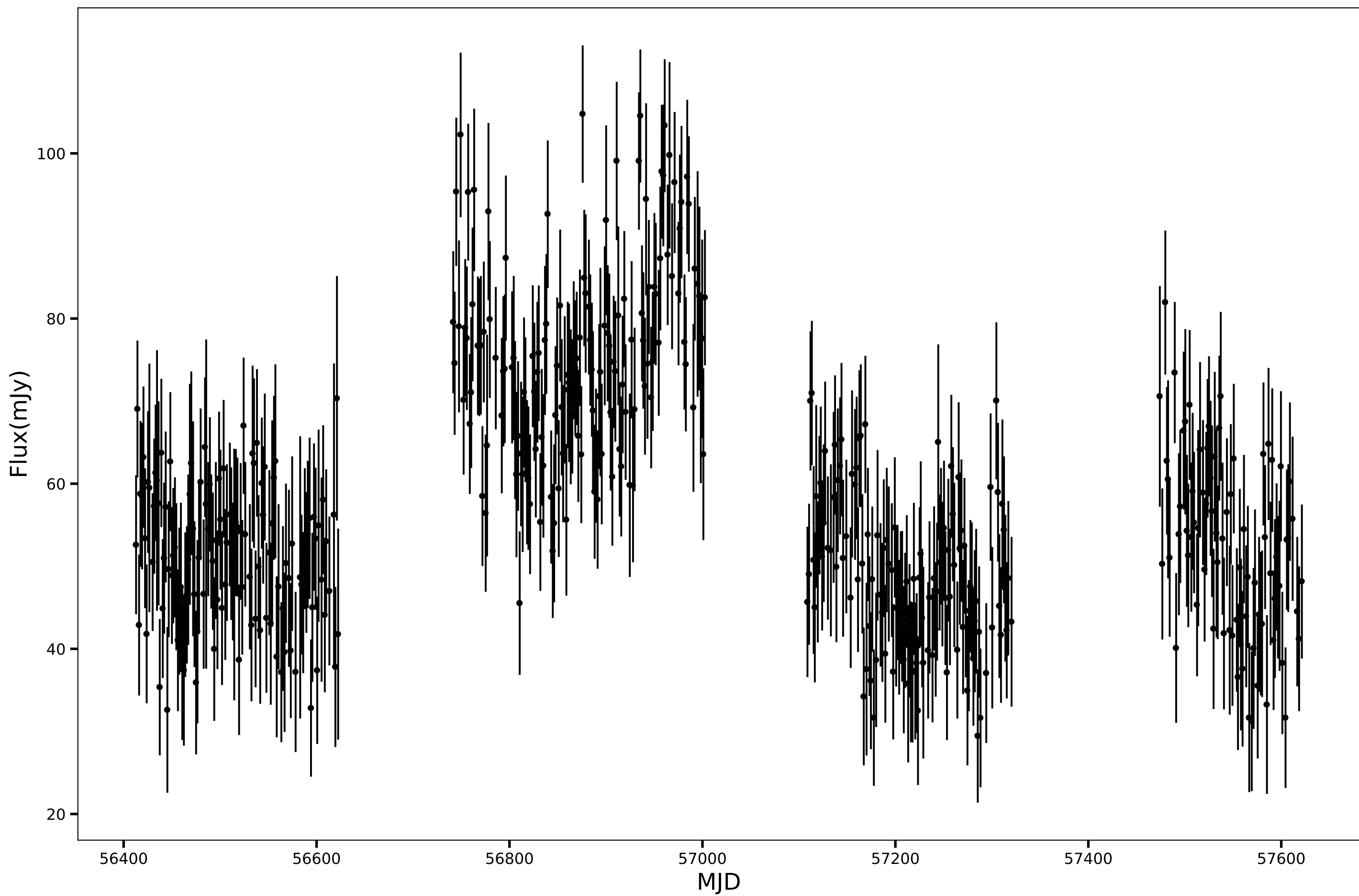
SPT-SJ223905-5526.0, RA=339.7745d, DEC=-55.4347d, mean_flux=58.25 (mJy), 150GHz
