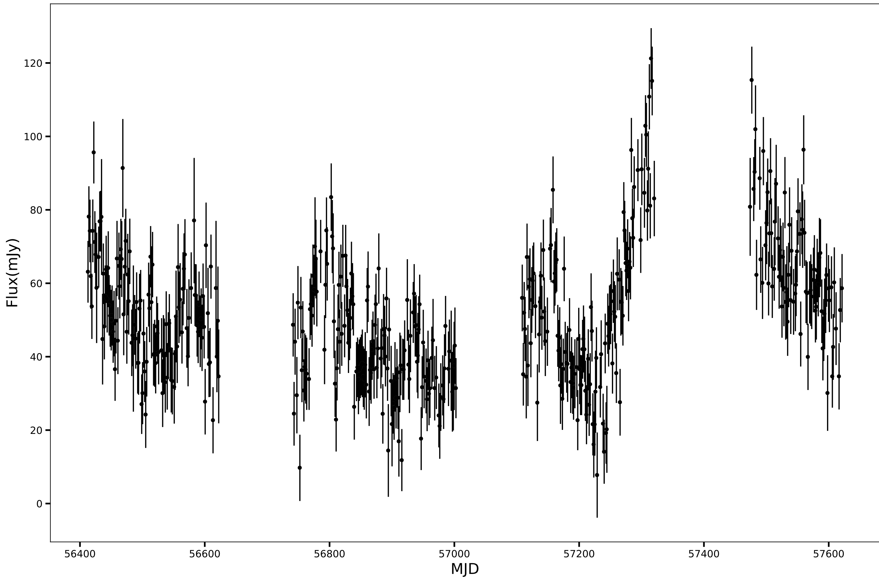
SPT-SJ223825-5114.3, RA=339.6050d, DEC=-51.2397d, mean_flux=51.30 (mJy), 150GHz
